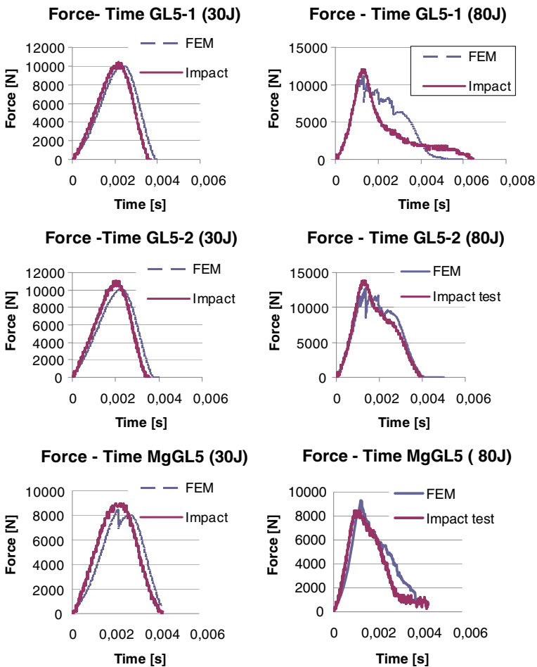
Fig. 11 Force-time histories, FEM and experimental results
