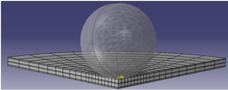
Fig. 1 Finite element model (mesh geometry). Dark layers are made of AL 2024-T3 or Mg AZ31B-H24 and bright layers are FM94/S2
