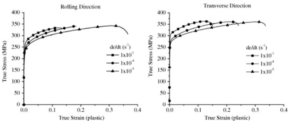
Fig. 2 Stress–strain behavior as a function of applied strain rates for rolling and transverse directions of AZ31B magnesium alloy [30]
