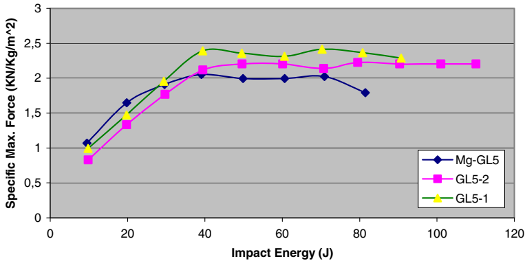
Fig. 6 Specific maximum force for the tested laminates
