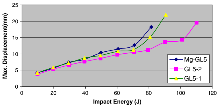
Fig. 7 Maximum displacements for the tested laminates
