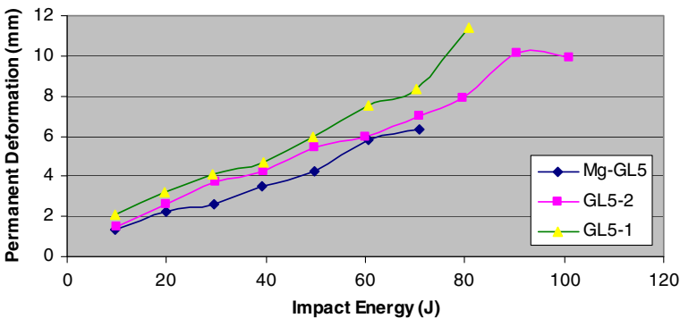
Fig. 9 Permanent deformations (maximum dent) for the tested laminates
