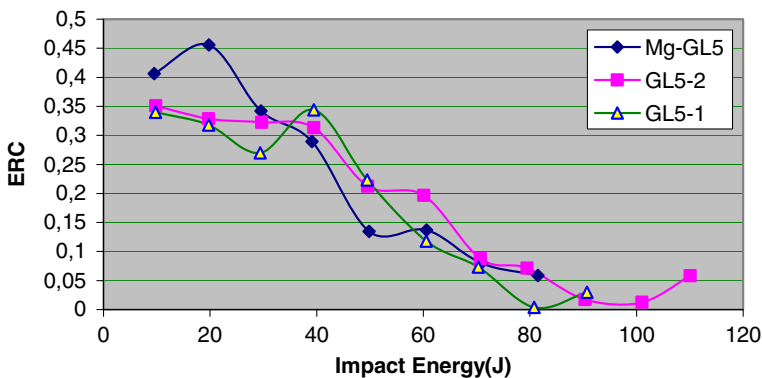
Fig. 3 ERC curves for the tested laminates
