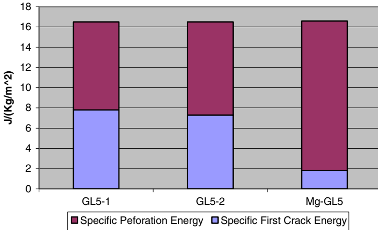
Fig. 4 Specific limit energies for the tested laminates
