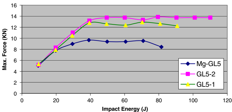
Fig. 5 Maximum impact forces for the tested laminates
