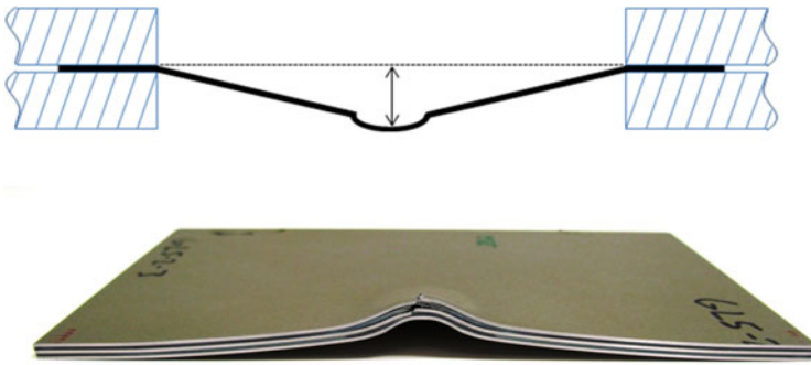
Fig. 8 The permanent deformation measurement
