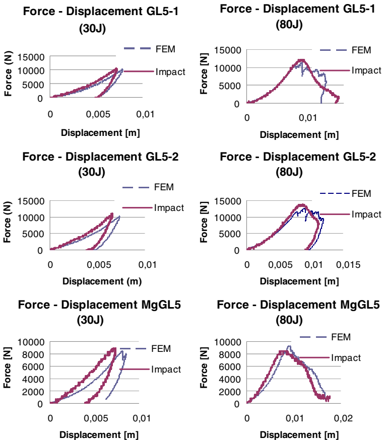
Fig. 12 Force-displacement curves, FEM and experimental results
