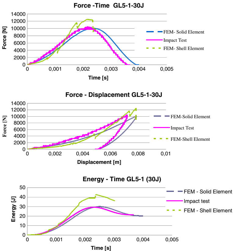
Fig. 13 Comparison of FE-predictions (energy-time) for two element types with the experimental data as reference
