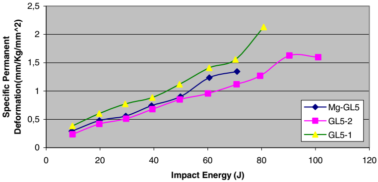
Fig. 10 Specific permanent deformations for the tested laminates
