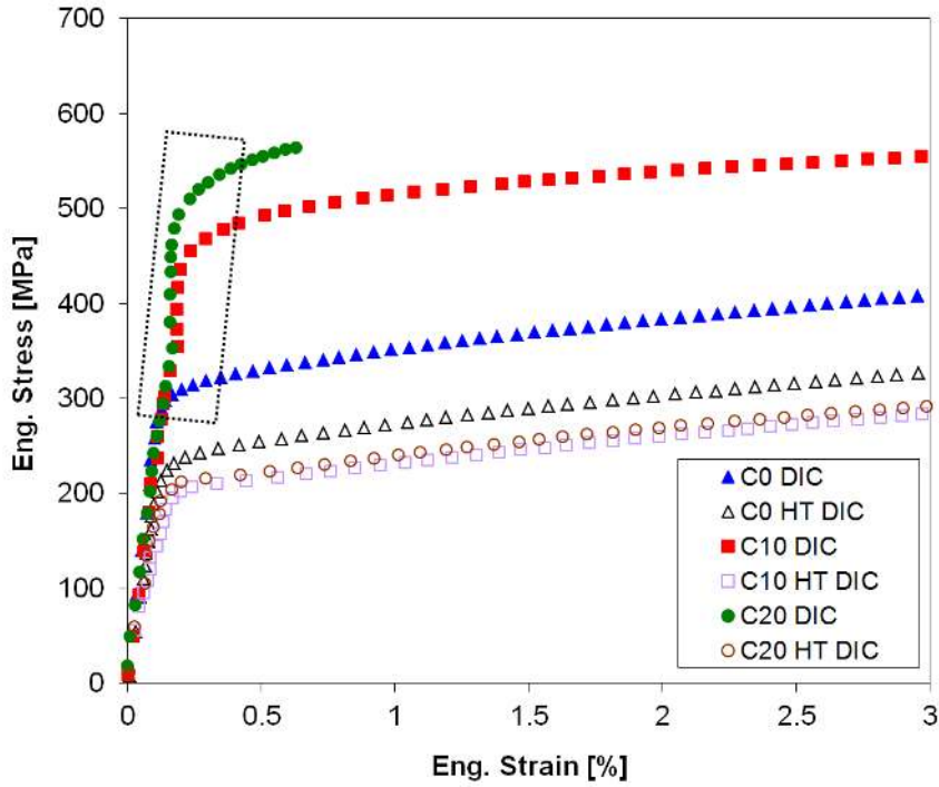
Fig. 9 Stress-strain data measured using DIC at 10mm from the WCL of cross-weld specimens.
