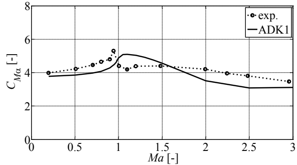
Fig. 4. Predicted values (ADK1) and experimental values (exp.) of derivative of pitching moment coefficient
