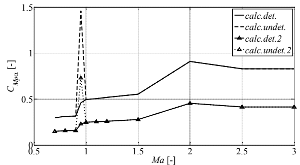
Fig. 6. Predicted values (ADK1) of derivative of Magnus moment coefficient [14]
