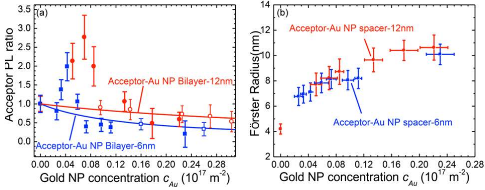
Figure 7. (a) PL ratio of the acceptor PL in a trilayer structure, I_{Acc, Tri} / I_{Acc, BL} , and the acceptor on Au NP structure, I_{Acc, Au} / I_{Acc} , as a function of the Au NP concentration. The trilayer samples with an acceptor-Au NP separation of t_{Acc-Au} = 6 nm (solid blue squares) and t_{Acc-Au} = 12 nm (solid red circles) have a fixed donor-Au NP separation, t_{Don-Au} = 3 nm. Data for the acceptor-Au NP bilayer samples with an acceptor-Au NP separation of t_{Acc-Au} = 6 nm (open blue squares) and t_{Acc-Au} = 12 nm (open red circles) are also shown. The solid lines show the calculated acceptor PL ratio for acceptor-Au NP bilayers with the same separations using the NSET model (equation 3). (b) The dependence of the extracted effective Förster radius for trilayer samples on the Au NP concentration. The acceptor-Au NP separations are t_{Acc-Au} = 6 nm (solid blue squares) and t_{Acc-Au} = 12 nm (solid red circles), with a fixed donor-Au NP separation, t_{Don-Au} = 3 nm.
