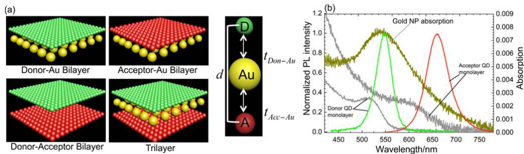
Figure 1. (a) Schematics of the trilayer, donor-acceptor bilayer and QD-Au NP bilayer reference structures. The PE spacer layer thickness is denoted by t , where t_{Don-Au} and t_{Acc-Au} correspond to the PE spacer layer thickness between the intermediate Au NP monolayer and the donor QD and acceptor QD monolayers, respectively. The donor-acceptor center-to-center distance is denoted by d . (b) Normalized PL spectra of a donor QD monolayer (green line) and acceptor QD monolayers (red line). Absorption spectra of both the QD monolayers (grey lines) and Au NP layer (yellow line) are also shown.
