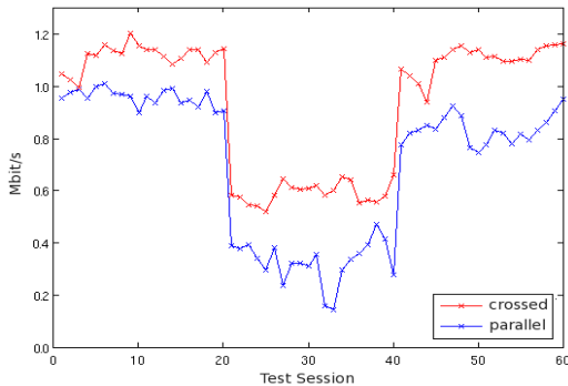
Figure 12. Goodput of Bluetooth under the interference of Wi-Fi.
