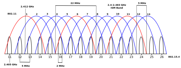
Figure 1. Channel Occupancy of 802.11 and 802.15.4 systems.
