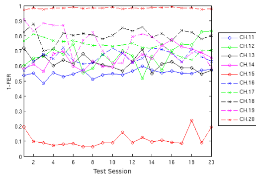
Figure 7. 1-FER of the first ten ZigBee channels under the interference of Wi-Fi channel 1 – crossed configuration.
