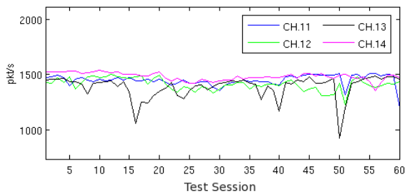
Figure 6. Goodput of Wi-Fi under the interference of ZigBee – crossed configuration.
