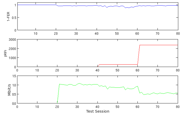
Figure 14. 1-FER of ZigBee (top) and goodput of Wi-Fi (center) and Bluetooth (bottom) – parallel configuration.
