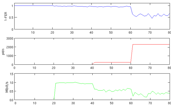
Figure 16. 1-FER of Zigbee (top) and goodput of Wi-Fi (center) and Bluetooth (bottom) – Wi-Fi-crossed configuration.
