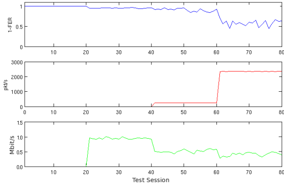
Figure 15. 1-FER of Zigbee (top) and goodput of Wi-Fi (center) and Bluetooth (bottom) – ZigBee-crossed configuration.
