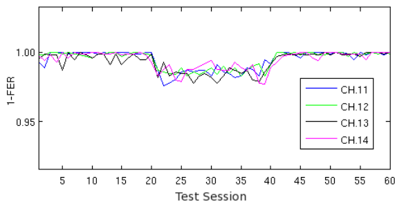
Figure 5. 1-FER of ZigBee under the interference of Wi-Fi – parallel configuration.
