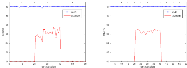
Figure 13. Goodput of Wi-Fi (in Mbit/s) under the interference of Bluetooth.
