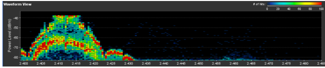
Figure 8. Spectrum of Wi-Fi activity on channel 1.
