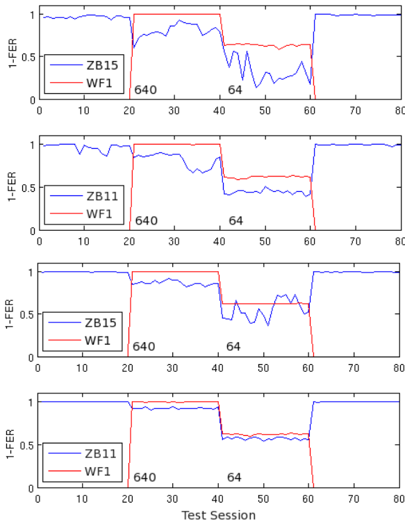
Figure 9. 1-FER of ZigBee (channels 11 and 15) under the interference of Wi-Fi (channel 1, varying payload size) for the crossed (top two) and parallel (bottom two) configurations.
