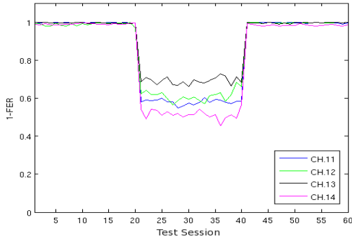
Figure 4. 1-FER of ZigBee under the interference of Wi-Fi – crossed configuration.
