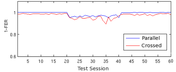
Figure 10. 1-FER of ZigBee under the interference of Bluetooth for both crossed and parallel configurations.
