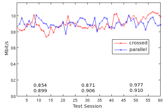
Figure 11. Goodput of Bluetooth under the interference of ZigBee for both crossed (red) and parallel (blue) configurations.
