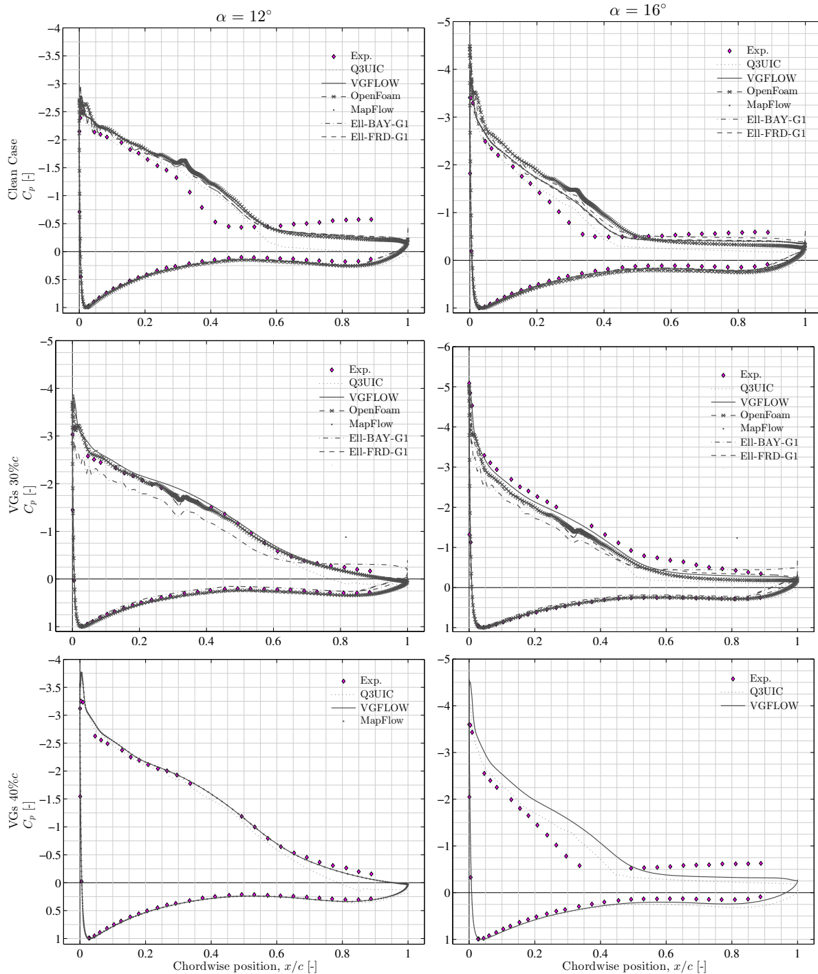
Figure 8: Pressure distributions for the NTUA T18 airfoil; C_p(x) for (Left column) \alpha = 12^\circ and (right column) \alpha = 16^\circ . Rows represent the Clean Case, VGs at 30% c and 40% c respectively. (Note different graph scale).
