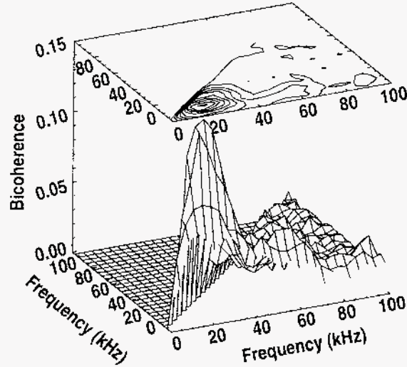
FIG. 6. Bicoherence spectrum between density fluctuations and derived velocity fluctuations, \hat{b}^2 = \frac{\langle n_{f_1} n_{f_2} v_{\theta} \rangle}{\langle n_{f_1} n_{f_2} \rangle \sqrt{\langle v_{\theta} v_{\theta}^* \rangle}} .
