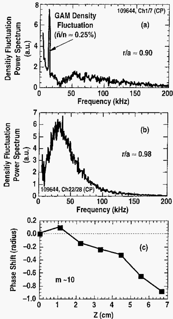
FIG. 7. (a) Density fluctuation near r/a=0.90 associated with the GAM poloidal velocity oscillation, showing measurable density or pressure perturbation, and (b) density fluctuation spectrum near r/a \approx 0.98 showing no apparent fluctuation; (c) poloidal phase shift of density perturbation showing finite m number ( m \sim 10 ).
