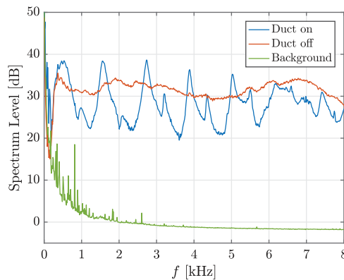
Figure 5. Averaged spectrum level over the microphones in the array for the omnidirectional source in red and the modified spectrum with the duct on in blue. The green line indicates the background spectrum with the source off.
