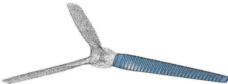
Figure 3. 3D scan of the propeller (black dots) and blade reconstruction in CATIA™.
