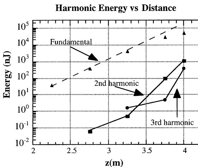
FIG. 2. Energy vs distance for the fundamental, 2nd and 3rd harmonics. The gain lengths for these are 19, 9.8, and 6.0 cm, respectively.
