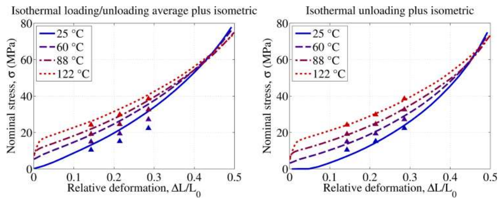
FIG. 9. Experimental characterization of the RC mechanical response. The lines represent the average response in cyclic isothermal tests. Triangular markers represent the interpolated force in isometric tests, at the same temperatures at which isothermal tests were conducted.
