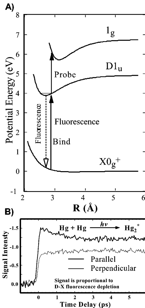
Figure 29. (A) FPAS experiment on Hg. The initial (binding) pulse forms \text{Hg}_2 in the D state; the depletion of the D \rightarrow X fluorescence is monitored, as probe causes excitation to the 1g state. The region of most probable excitation from the ground state is shown in the inset. (B) FPAS transients showing depletion of the D \rightarrow X fluorescence, as shown in A. Data are for the binding and probe lasers polarized parallel or perpendicular to one another. Note the rotational dephasing of the initial anisotropy. (Reprinted with permission from ref 525. Copyright 1995 Elsevier Science B. V.).
