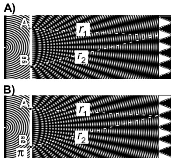
Figure 1. Schematic simulation of Young's double-slit experiment in which the distance between the slits A and B is equal to 10 \lambda . (A) A plane wave is diffracted by a small pinhole, and the resulting wave encounters two small slits. The emerging light interferes and is detected at the screen. (B) Same as above, but in slit B a phase delay of \pi is introduced. Notice that this delay shifts the intensity pattern on the screen from a maximum to a minimum, and vice versa.
