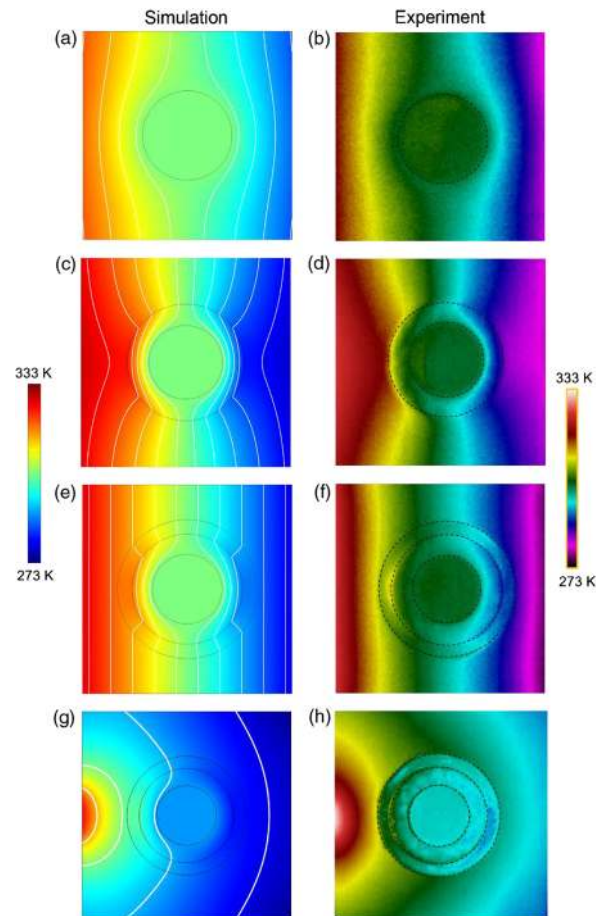
FIG. 2 (color online). Simulated and measured temperature distributions for the steady state. (a),(b) First reference structure. (c),(d) Second reference structure. (e),(f) The proposed bilayer cloak with a = 6 , b = 9.5 , and c = 12 mm. (g),(h) The proposed bilayer thermal cloak in the presence of a point heat source, emitting cylindrical heat fronts. Isothermal lines are also represented with white color in the panel.
