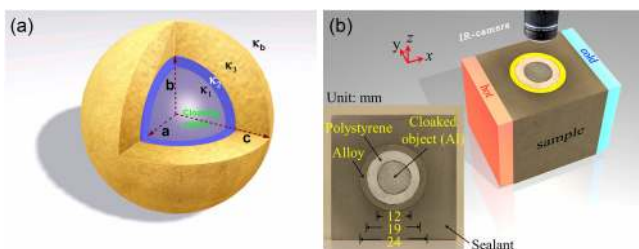
FIG. 1 (color online). (a) Schematic illustration of the 3D and 2D bilayer thermal cloak with naturally available materials. (b) Experimental setup for the 2D bilayer thermal cloak. The inset shows the cross section of the experimental sample.
