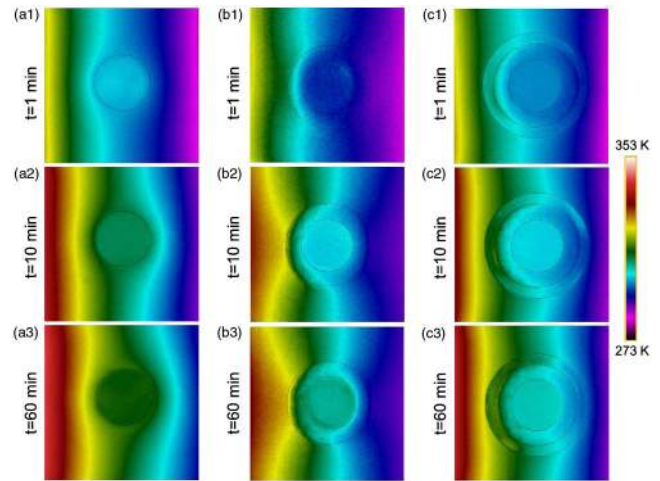
FIG. 3 (color online). Experimental transient temperature distributions at different times t = 1, 10, 60 min. (a) Results for the first reference structure of Fig. 2(b). (b) Results for the second reference structure of Fig. 2(d). (c) Results for the bilayer cloak of Fig. 2(f). Obviously, both bilayer cloak and insulation coating can make the object colder than the bare object. However, only bilayer cloak can restore isothermal lines exactly without distortion as if nothing were there.
