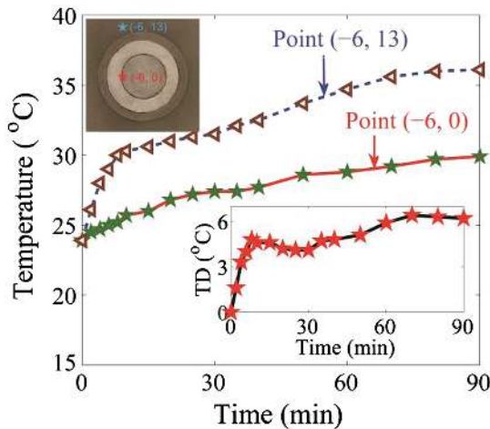
FIG. 4 (color online). Measured time-dependent temperature for test points at (-6,0) and (-6,13) mm. Points (-6,0) and (-6,13) denote the cloaking region and the surrounding (external region) respectively, which have been illustrated in the upper left inset. Lower-right inset shows the temperature difference between the two test points.
