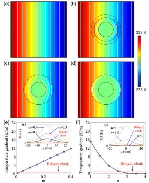
FIG. 5 (color online). Temperature distributions and quantitative comparison for different thermal cloaking schemes. (a) A pure background. (b) Bilayer thermal cloak proposed in this Letter. (c) AI thermal cloak with m = 0.2 . (d) AH thermal cloak with n = 3 . (e) Temperature gradient at (0,0) for AI thermal cloak with different m . The inset shows the temperature deformation of the AI thermal cloak with different m . (f) Temperature gradient at (0,0) for the AH thermal cloak with different n . Inset shows the temperature deformation of the AH thermal cloak with different n . Isothermal lines are also represented with white color in the panel.
