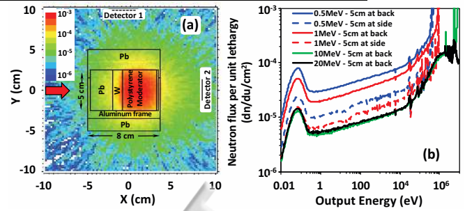
FIG. 2. (a) The design of the moderator superimposed on the neutron (in the range 1eV-1keV) flux distribution across the mid-plane of the moderator, obtained from MCNPX simulation for 1 MeV neutrons entering the moderator from the left side (shown by red arrow). (b) Comparison between neutron spectra at the two detectors, detector-1 and detector-2 respectively (shown in (a)), placed 5 cm away from the side and exit faces of the moderator for different incident neutron energies as obtained from MCNPX simulations.
