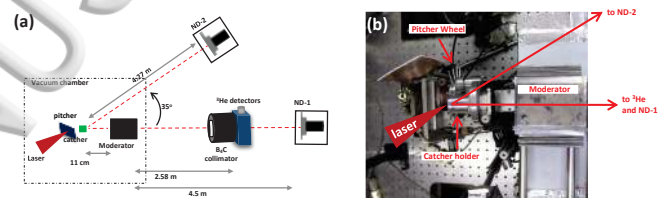
FIG. 1. (a) Schematic of the experimental setup (figure not to scale). (b) Image of the setup inside the interaction chamber. The fast neutrons were generated by nuclear reactions in the catcher target induced by the MeV ions accelerated from the laser irradiated pitcher target. ND-1 and ND-2 are EJ232Q scintillator detectors, placed inside lead and plastic housings, employed in ToF mode to diagnose the fast neutron spectra[18]. Epithermal neutrons produced by the moderator were diagnosed by the ^3\text{He} proportional counters employed in ToF mode, placed behind a B 4 C collimator.
