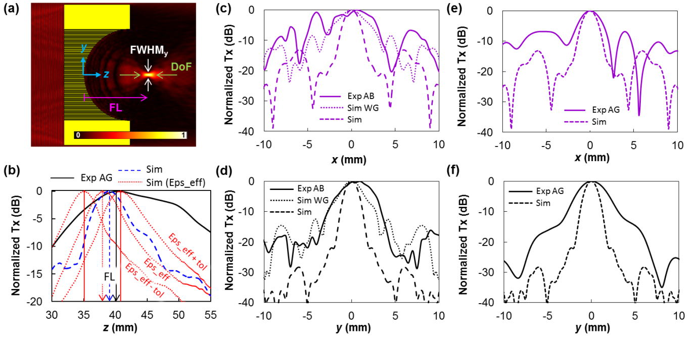
Fig. 4. (a) Numerically-computed magnitude of the electric field normalized to the maximum on the yz -plane at the working frequency f_0=144 GHz. (b) Normalized transmission along the z -axis for x=y=0 mm at f_0 where the focal length is marked with vertical arrows. Continuous line (Exp AG) represents measured values with Agilent VNA setup, dotted line (Sim) simulated values of the full lens and dashed line (Sim(Eps_eff)) simulated values of the lens formed by homogenous material. (c, e) Normalized transmission at f_0 along the x -axis and (d, f) along the y -axis at the FL. Exp AB and Exp AG represent experimental results obtained with the AB Millimetre and Agilent VNA setup, respectively. Sim WG and Sim represent simulation results with and without the modeling of the detector, respectively.
