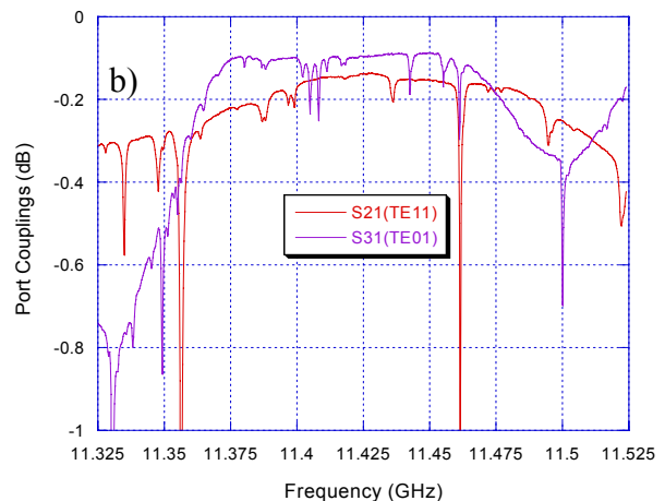
Figure 4: a) Mode stripper and b) cold test measurements.
