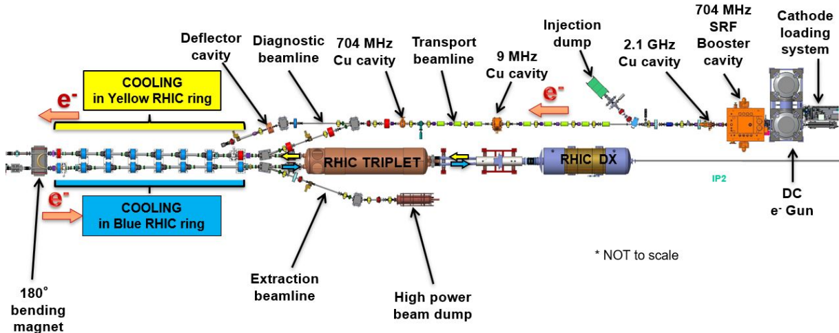
FIG. 1: Layout of the LEReC accelerator (not to scale).
