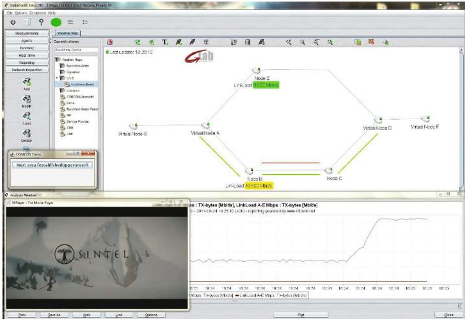
Fig. 8. VoD service running and serving an increasing number of clients
