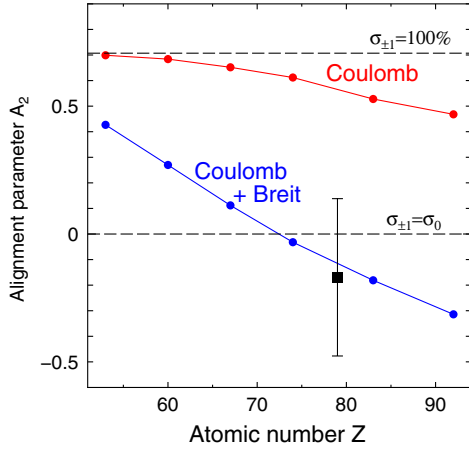
FIG. 3 (color online). Alignment parameter \mathcal{A}_2 for intermediate state [1s2s^22p_{1/2}]_1 in DR of Li-like ions. The present result for Au ( Z = 79 ) is shown by the black square. Theoretical values taken from Ref. [8] are plotted as red dots (Coulomb interaction only) and blue dots (with Breit interaction).
