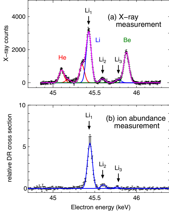
FIG. 2 (color online). (a) K x-ray intensity plotted as a function of electron beam energy for the KL_{12}L_{12} resonance region of highly charged Au ions. The background corresponding to radiative recombination is subtracted. The labels represent the charge state responsible for the DR process that led to x-ray enhancement. (b) Relative DR cross section [Eq. (4)] of Li-like Au obtained from ion-abundance measurement. The Gaussian functions fit to the experimental data are also shown by solid lines for both (a) and (b).
