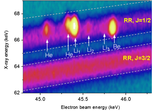
FIG. 1 (color online). X-ray spectra from the KL_{12}L_{12} DR of highly charged Au ions. X-ray counts are plotted as a brightness of color as functions of electron beam energy (horizontal axis) and x-ray energy (vertical axis). Bright spots correspond to x-ray enhancement due to the DR. The charge state responsible for each spot is indicated by labels. For the Li-like ion, which is of interest in the present study, the intermediate and final states are listed in Table I.
