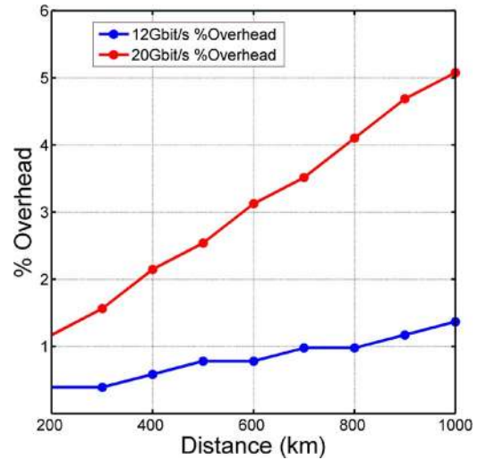
Fig. 10. Cyclic prefix for the 12- and 20 -Gbit/s systems.
