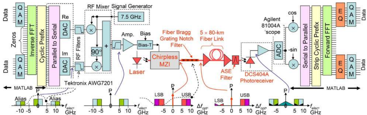
Fig. 6. 10 Gbit/s RF electrical upconverted system.
