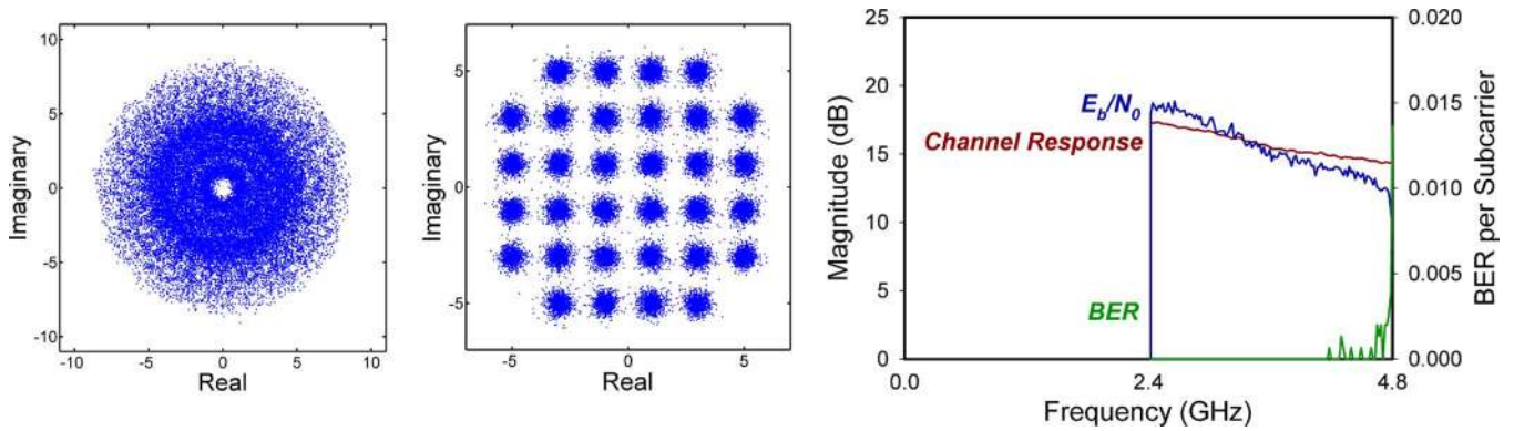
Fig. 4. Results for 12-Gbit/s colorless system using digital Hilbert transform to generate single sideband signal. Unequalized constellation. Equalized constellation. Channel response E_b/N_0 and BER.
