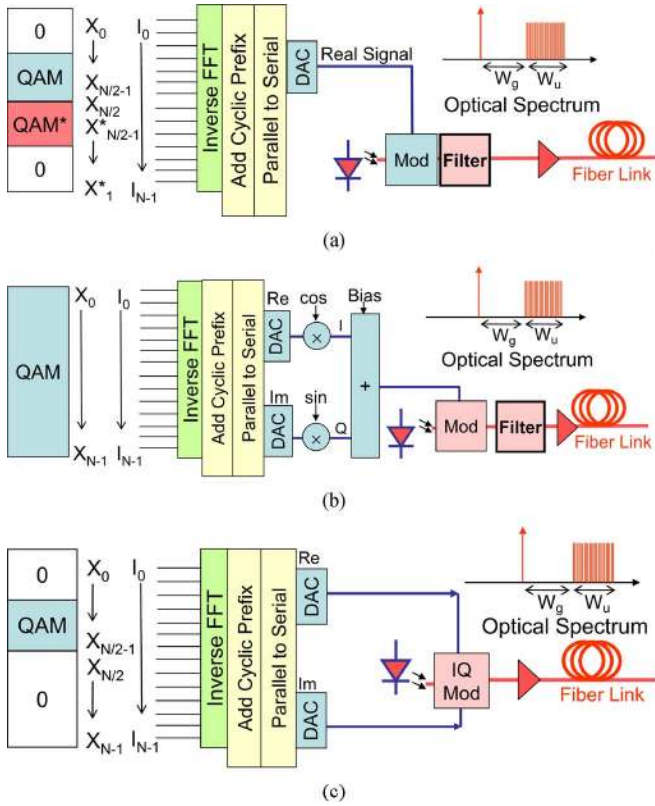
Fig. 1. DD-OOFDM transmitters: (a) using Hermitian symmetry and an optical filter; (b) using upconversion and an optical filter; (c) using a frequency domain Hilbert transform.
