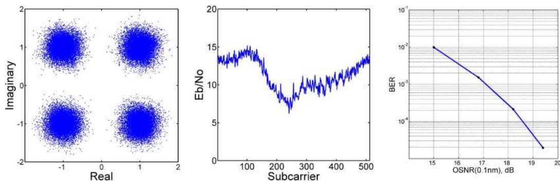
Fig. 7. Results for 10-Gbit/s system using RF upconversion. Equalized constellation. E_b/N_0 versus Subcarrier – High frequencies in middle subcarriers. BER versus OSNR.
