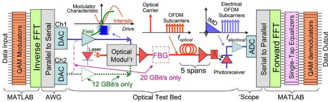
Fig. 3. Schematic of the two digital baseband electrical systems: 12 and 20 Gbit/s.
