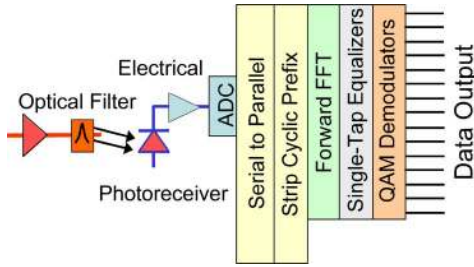
Fig. 2. DD-OOFDM direct detection receiver.
