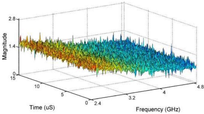
Fig. 8. Channel stability.
