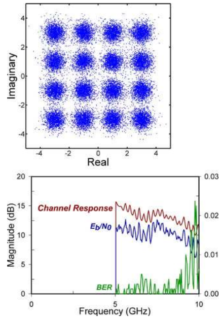
Fig. 5. Results for 20 Gbit/s digital system. Equalized constellation channel response, E_b/N_0 and BER.
