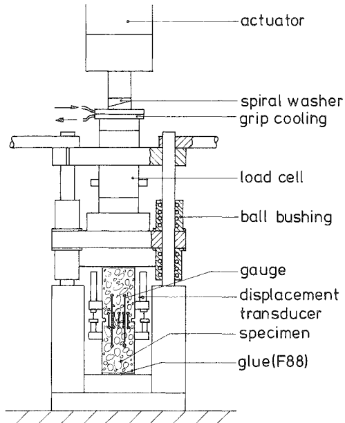
Fig. 2. View of the testing equipment.
