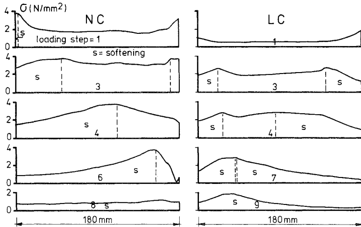
Fig. 11. Calculated stress distribution of wide specimens.
