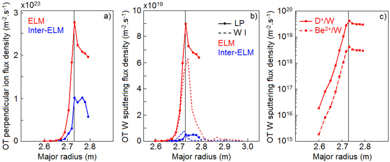
Figure 9. (a) OT perpendicular ion flux density profile from LP, (b) OT total W sputtering flux density profile from WI spectroscopy (dashed curves) and LP (plain curves) due to ELM (red curves) and inter-ELM (blue curves) and (c) contribution from D^+ (plain curve) and Be^{2+} (dashed curve) to OT W sputtering flux density profile.
