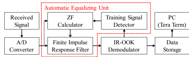
Fig. 10: Block diagram of the developed receiver
