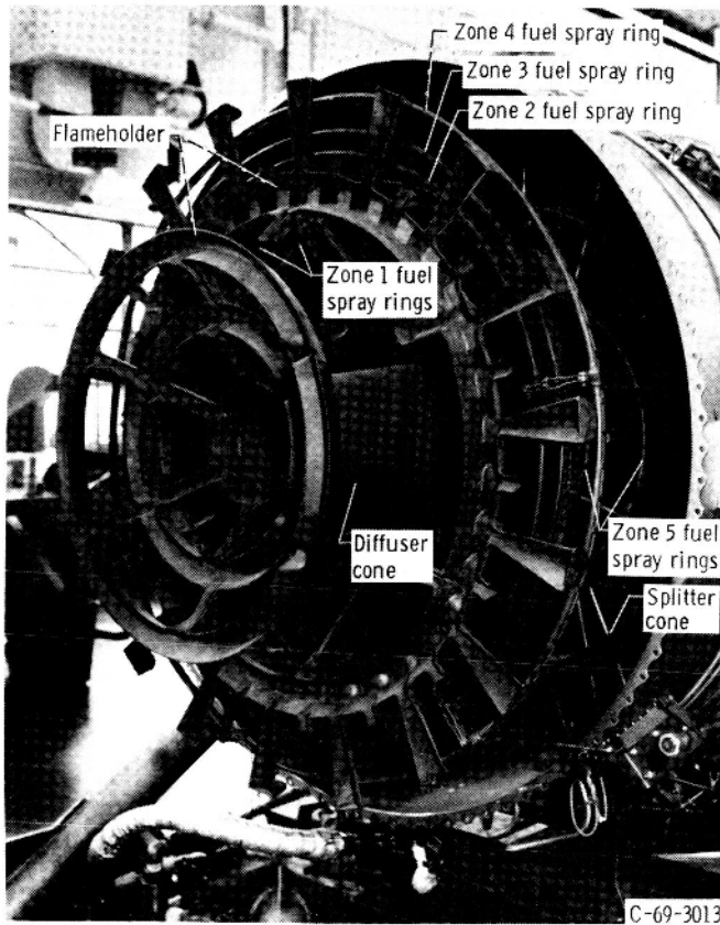
Figure 3. - Afterburner flameholder and spray rings assembly. View looking upstream.
