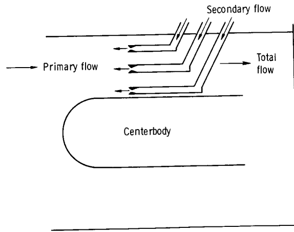
(b) Schematic drawing of jet array.
