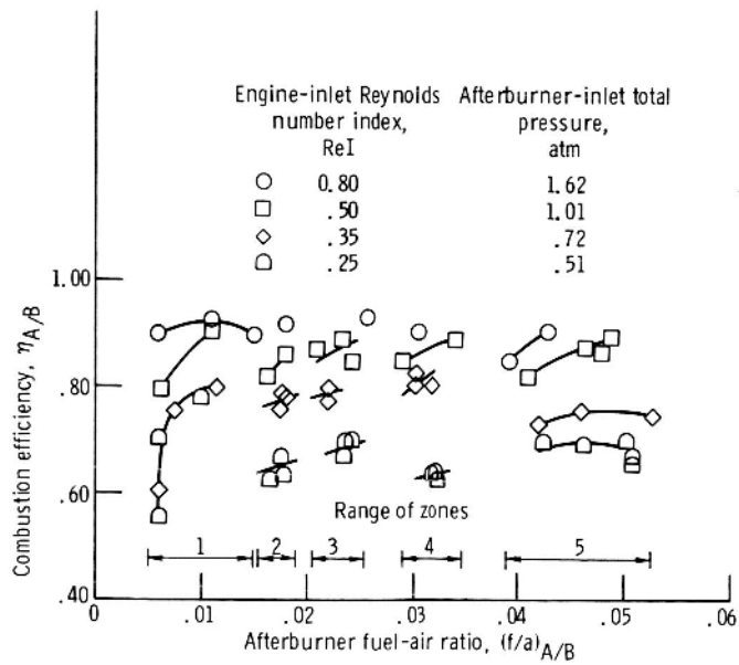
Figure 6. - Effect of afterburner pressure level and fuel-air ratio on afterburner combustion efficiency with steady-state distortion-free engine-inlet flow. Engine-inlet temperature, 16^{\circ} C.
