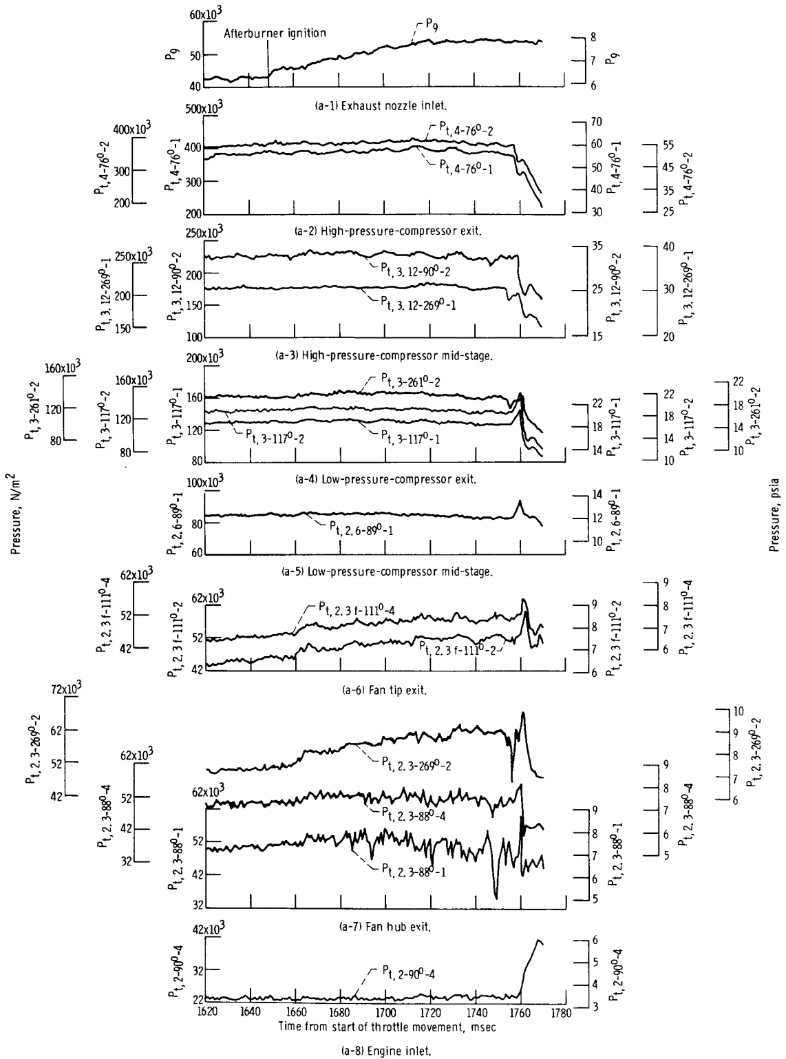
(a) Throttle burst from Military to Maximum throttle position.
