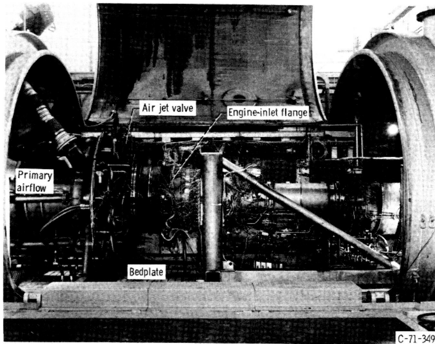
Figure 5. - Afterburning turbofan with air jet system installed in altitude test chamber.
