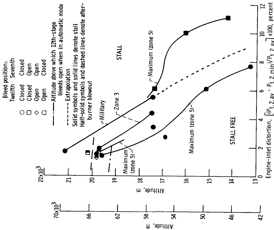
Figure 15. - Altitude-distortion limits at fixed throttle positions. Air jet 180° distortion; simulated flight Mach number, 1.4; undistorted inlet recovery, 0.978.
