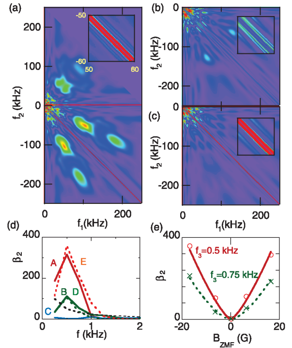
FIG. 3 (color). Coupling of zonal field and turbulence. Bicoherence analysis using Gabour's wavelet to show the existence of a linkage between zonal field and turbulence. Here the analysis adopts the conditional average to take into account the dependence of the coupling on the zonal field phase. Bicoherence diagrams of (a) phase A, (b) phase C, and (c) phase E. The insets are expanded views of a frequency range of 50 < f_1 < 60 kHz and -60 < f_2 < -50 kHz. (d) Total bicoherences in the frequency range below 2 kHz for all five phases. The dashed line shows an estimator giving a rough criterion of convergence. (e) The total bicoherence as a function of the averaged amplitude of the zonal field for the five phases.
