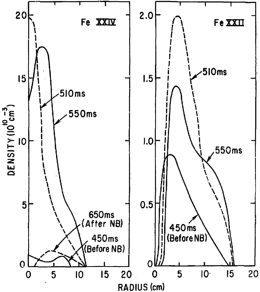
Fig. 6. Radial profiles of FeXXIV and FeXXII ion densities, corresponding intensity profiles from Fig. 5.
