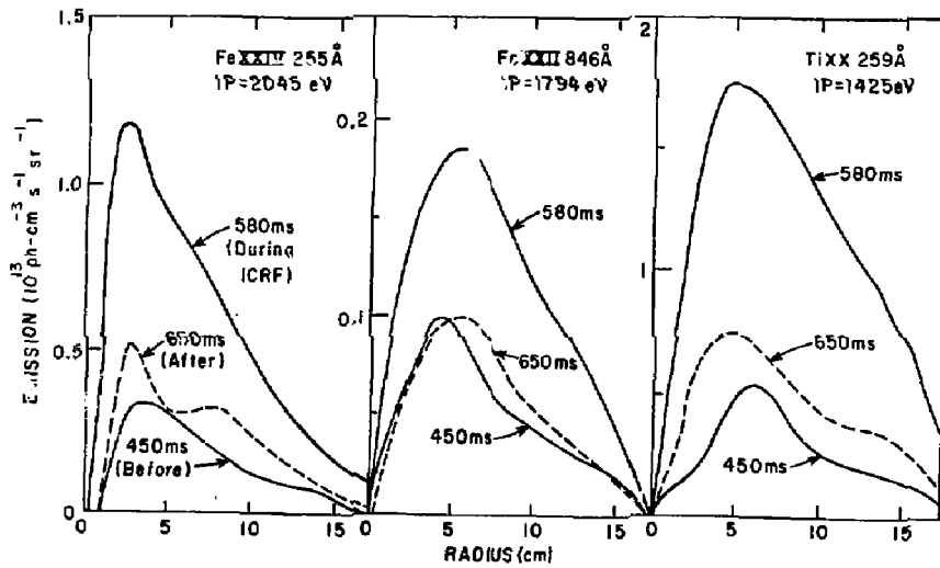
796571 Fig. 7. Time evolution and radial distribution of FeXXIV, FeXXII and TiXX line intensities during an ICRF heating experiment.
