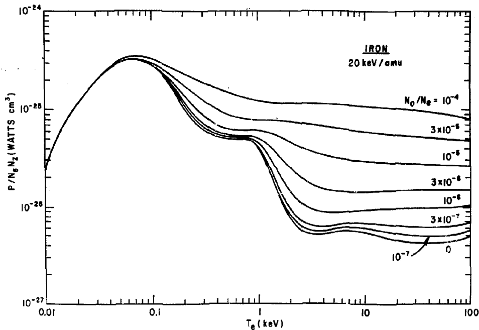
796570 Fig. 2. Emissive power per ion atom in a plasma at electron temperature T_e , with coronal equilibrium ionization balance modified by charge exchange recombination due to different neutral hydrogen to electron density ratio, N_0/N_e .
