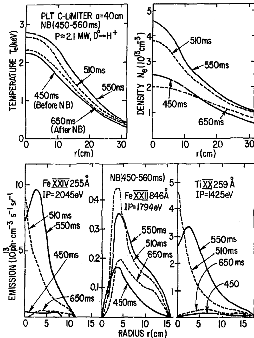
Fig. 5. Radial profiles of FeXXIV, FeXXII, and TiXX line intensities and the electron temperature and density before (450 ms) during (510 ms, 550 ms) and after (650 ms) neutral beam injection.
