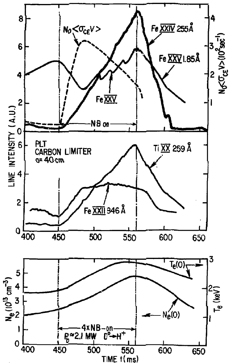
796411 Fig. 3. Time evolution of FeXXIV, FeXXV, FeXXII and TiXX line intensities during neutral beam injection. Dashed curve represents rate of charge exchange of FeXXV and D^0 . Central electron temperature T_e(0) and density N_e(0) are shown in lower part of the figure.
