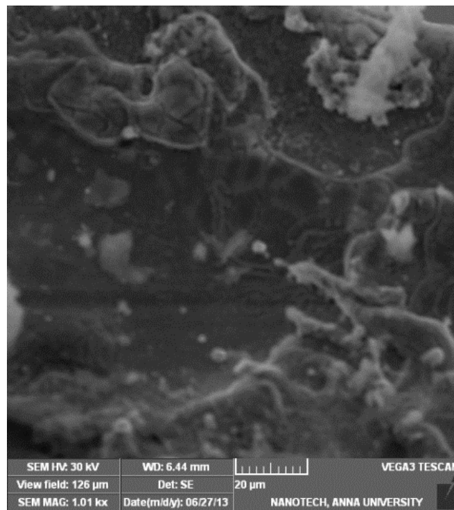
Fig. 8. Microstructure of the cut section of the bellows at the crest
