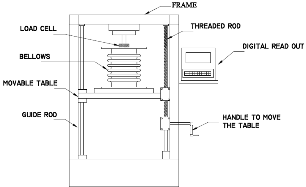
Fig. 4. Set up for Spring Rate Testing of the Hydroformed bellows.
