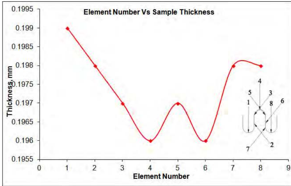
Fig. 3.Thickness Distribution of the convolution
