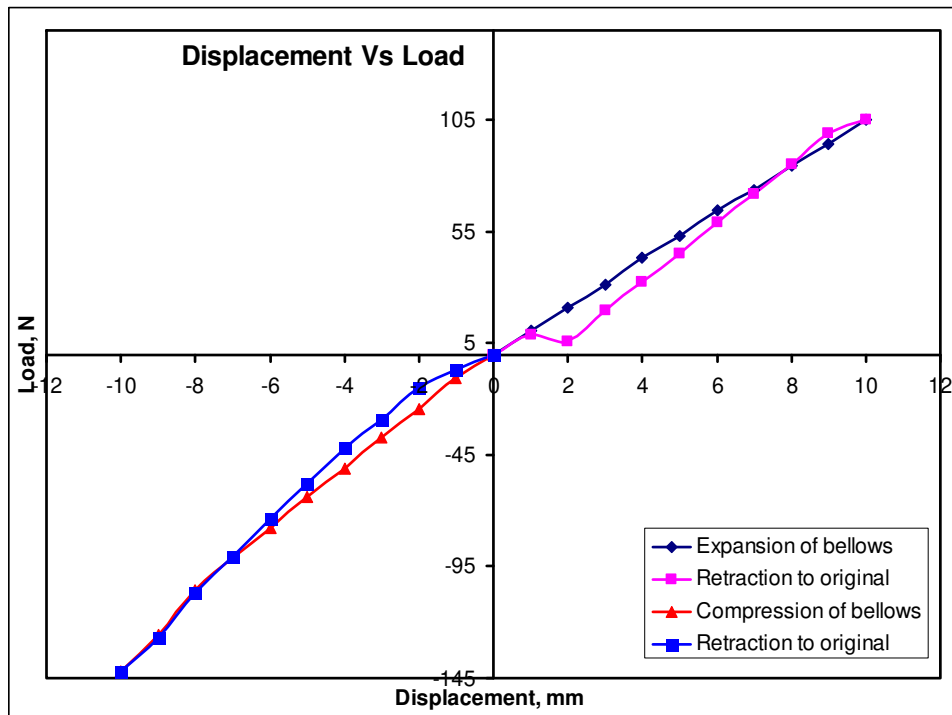
Fig. 5. Spring Rate of the Hydroformed bellows.
