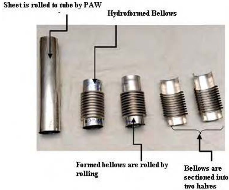
Fig. 1. Forming of Bellows
