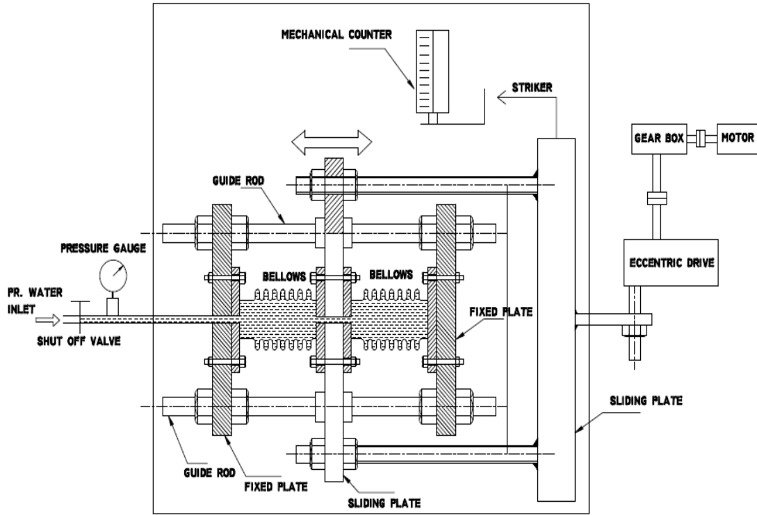
Fig. 6.Set up for Life Cycle Testing
