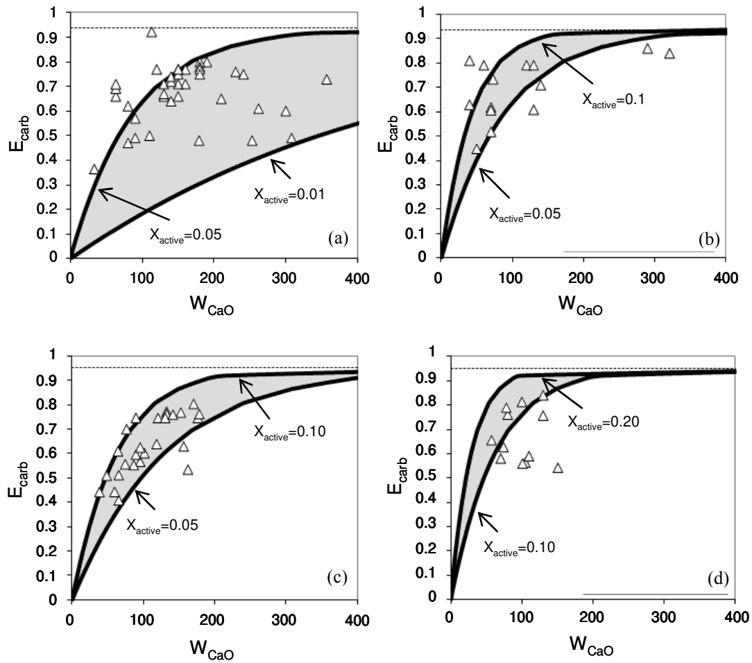
Figure 8. Capture efficiency as a function of the total CaO inventory in the carbonator. (Average values of tendency lines. Upper graphs: T_{\text{carb}}=636^{\circ}\text{C} , u=2\text{ m/s} , v_{\text{CO}_2}=0.11 , \phi_e=1.0 ; Lower graphs: T_{\text{carb}}=654^{\circ}\text{C} , u=3\text{ m/s} , v_{\text{CO}_2}=0.18 , \phi_e=1.0 ).
