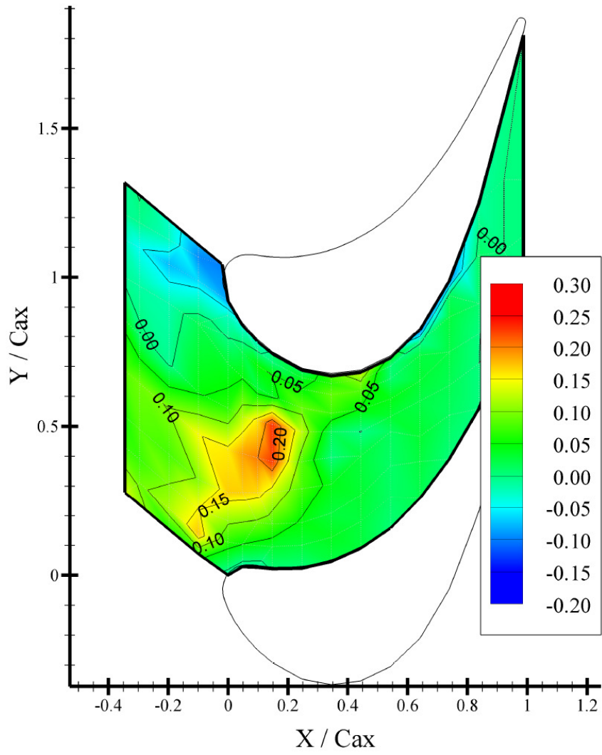
Figure 88. Endwall Adiabatic Film Cooling Effectiveness Contours for Differenced (Dolphin minus Shark Nose) Endwall Results with a Heated Approach Flow at 0.5% Leakage MFR
