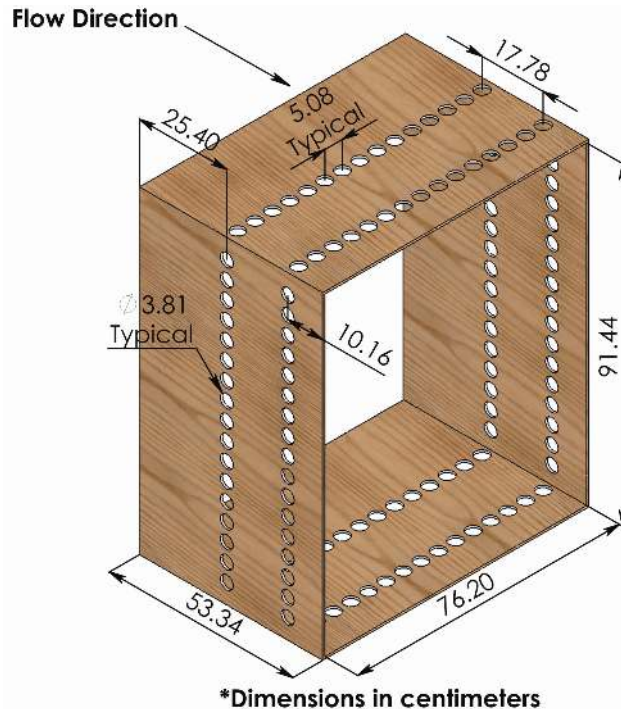
Figure 12. Turbulence Generator Cross Flow Walls
