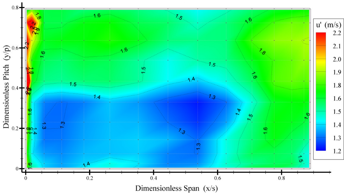
Figure 50. Approach Flow Distribution of u' ( x/C_{ax}=-0.58 )
