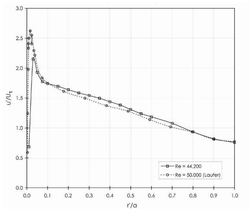
Figure 33. RMS of Turbulent Fluctuations in Fully-Developed Pipe Flow
