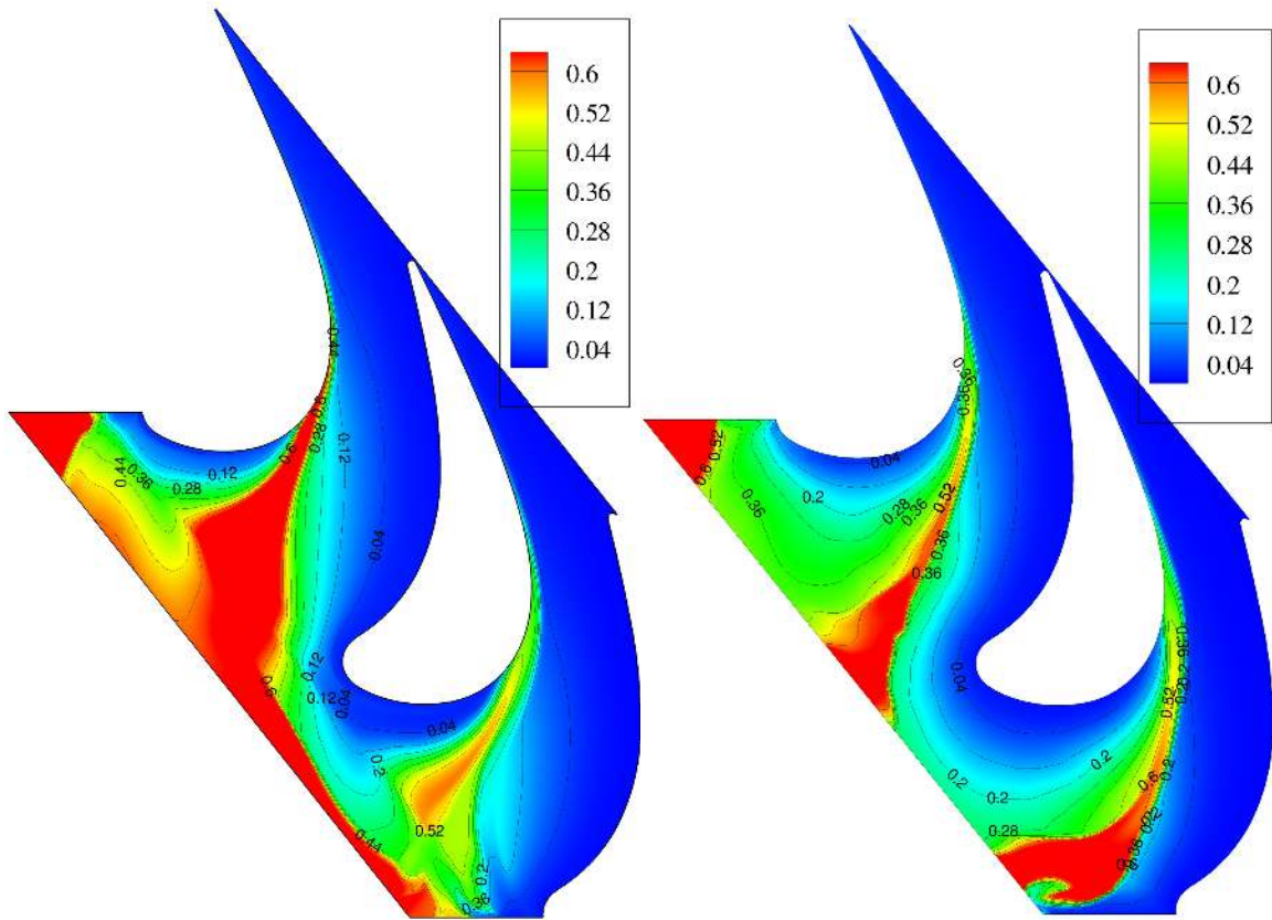
Figure 104. 3D CFD Results for Endwall Adiabatic Effectiveness on Dolphin Nose (Left) and Shark Nose (Right) Endwalls at Leakage MFR=1.0%
