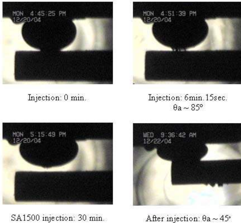
Figure 40: Depiction of Drop Movement During Surfactant Injection (Nonionic Surfactant A at 1500 ppm, 700 psi and 82^\circ\text{F} , Yates Live oil/Brine/Dolomite)
