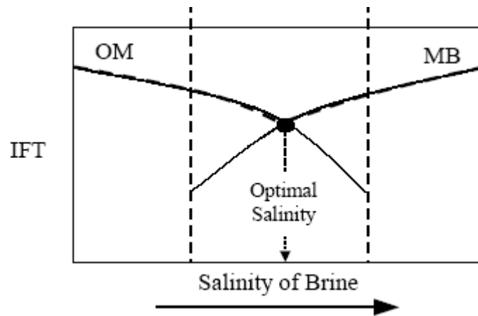
Figure 18: Optimal salinity in oil recovery [5]
