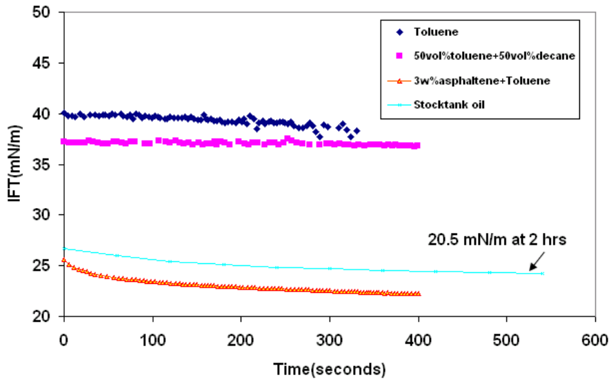
Figure 14: Dynamic Interfacial Tension of Different Oil Components in Deionized Water at Ambient Conditions using the Ambient Optical Cell
