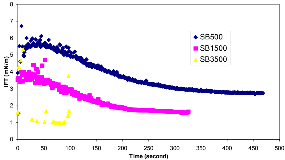
Figure 26: The Effect of Anionic Surfactant on Interfacial Tension of Yates Live Oil against Yates Brine at Reservoir Conditions (82°F & 700 psi)
