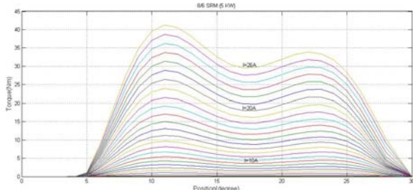
Fig. 6: Torque characteristics
