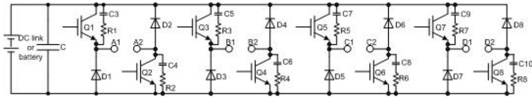
Fig. 3: Four-phase power converter
