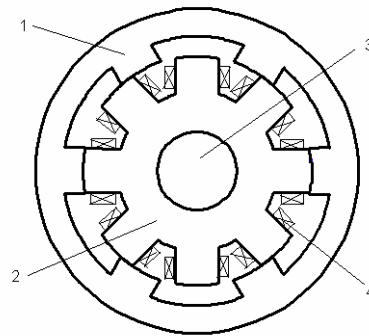
Fig. 1: Construct of in-wheel SRM (1-rotor; 2-stator; 3-shaft; 4-winding)
