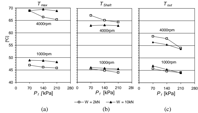
Fig. 10 – Influence of the oil supply pressure on (a) the maximum temperature at the bush-film interface, (b) the mean shaft-film interface temperature and (c) the oil outlet temperature ( T_i = 40^\circ\text{C} ).
