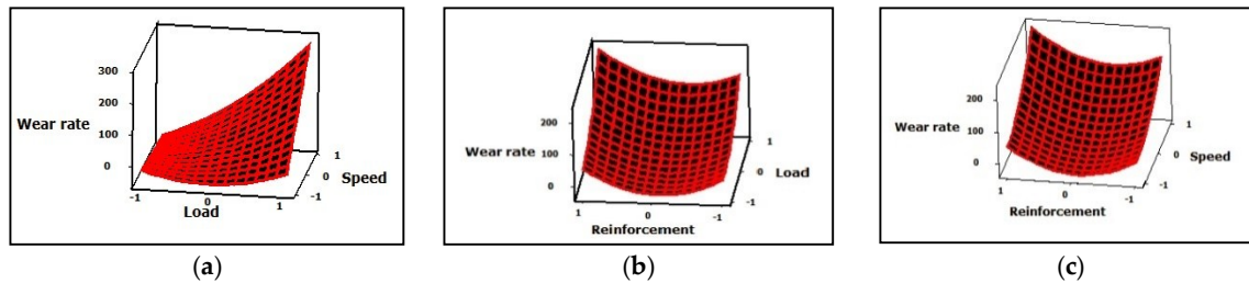
Figure 4. (a) Variation of wear rate with speed and load; (b) Variation of wear rate with load and reinforcement; (c) Variation of wear rate with speed and reinforcement.
