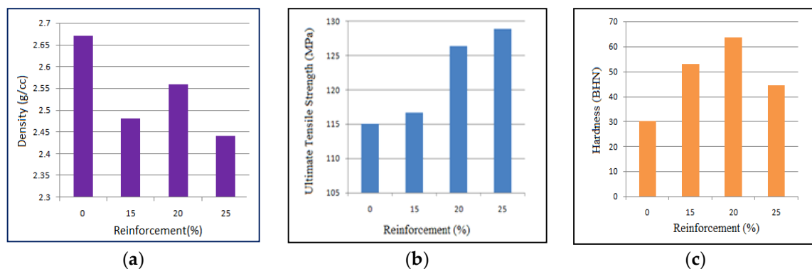
Figure 3. (a) Variation of density with reinforcement (b) Variation of tensile strength with reinforcement (c) Variation of hardness with reinforcement.
