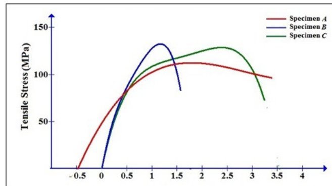
Figure 1. Stress-strain curve for specimens A, B, and C.
