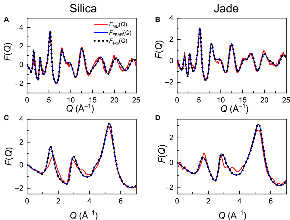
Fig. 1. Measured and simulated total reduced structure factors. F(Q) of (A and C) silica and (B and D) Jade glasses. The neutron experimental data are compared with simulation data obtained by FEAR and MD. In both cases, F(Q) derived by FEAR simulation (blue solid curves) matches well with neutron F(Q) (black dot curves), while significant discrepancy is observed for those of MD simulation (red solid curves), especially in low- Q region ( Q < 4 \text{ \AA}^{-1} ) as shown in (C) and (D).
