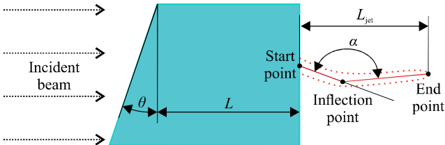
FIG. 1. Scheme of the PH formation behind ADP.
