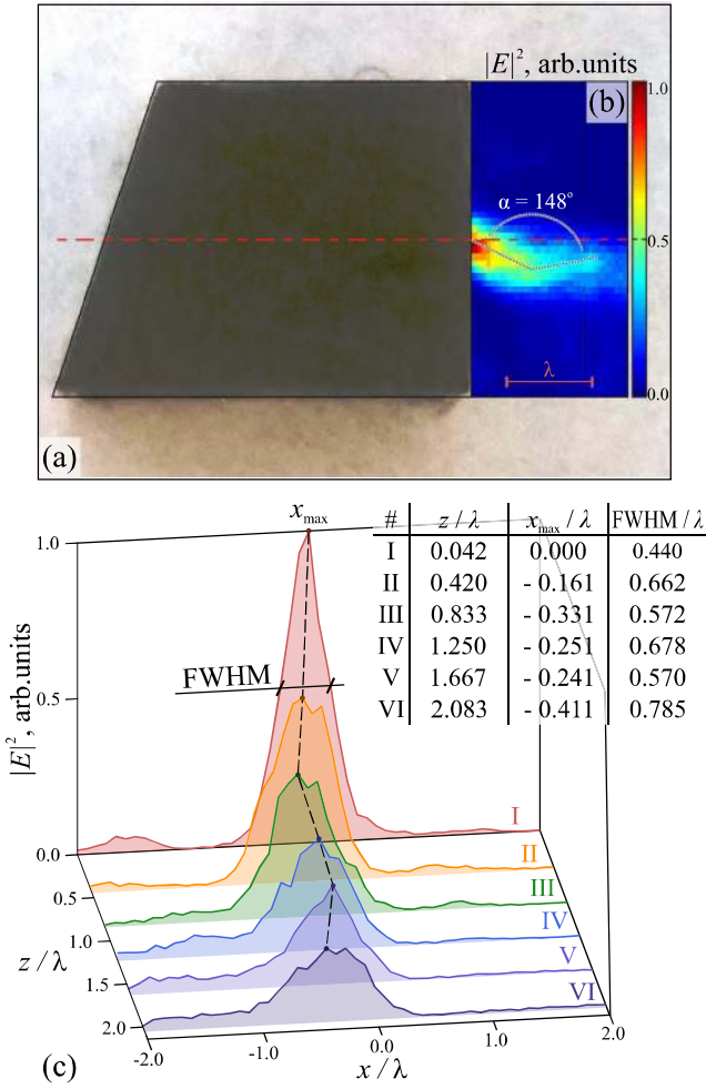
FIG. 4. Experimental visualization of a PH with the parameters from Fig. 2(e): (a) a photo of ADP made of TPX; (b) THz field intensity |E|^2 , at the shadow side of a particle illustrating the PH effect; (c) cross-sections of the observed PH. In (c), a table-inset shows parameters of the PH cross-sections.
