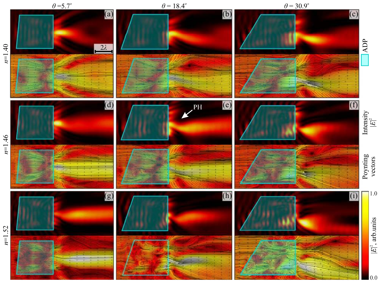
FIG. 2. Numerical analysis of the PH formation behind ADP, featuring the rib length of L = 4\lambda and different refractive indices n and prism angles \theta : (a)–(c) n = 1.40 and \theta = 5.7^\circ , 18.4^\circ , and 30.9^\circ ; (d)–(f) n = 1.46 and \theta = 5.7^\circ , 18.4^\circ , and 30.9^\circ ; (h)–(i) n = 1.52 and \theta = 5.7^\circ , 18.4^\circ , and 30.9^\circ . In each panel, the top image represents the EM field intensity |E|^2 , while the bottom image shows time-averaged Poynting vectors. The most pronounced PH is observed in panel (e).
