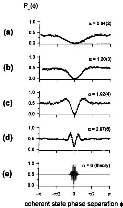
Figure 8. P_1(\phi) interference signal with increasing values of |\alpha| . The data are fitted to equation (10), yielding \alpha = 0.84, 1.20, 1.92 and 2.97 . The fit in curve (d) includes a term to account for the loss of contrast.
