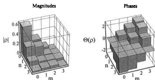
Figure 10. Experimental amplitudes \rho_{nm} and phases \Theta(\rho_{nm}) of the number state density matrix elements of a |\beta| \approx 0.67 coherent state. The state was displaced by |\alpha| \approx 0.92 , for N = 4 in equation (14).
