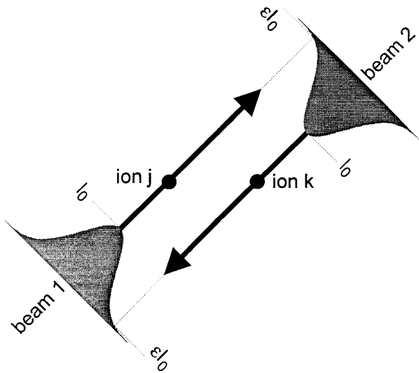
Fig. 5: Differential AC Stark shifting of neighboring ions. Equal intensity counter propagating beams 1 and 2 are centered on ions j and k , respectively. A fraction \epsilon of the peak intensity I_0 of each beam is applied to the other ion. This results in a differential AC Stark shift of ions j and k , allowing the possibility of individually accessing the ions by tuning the frequency of the laser beams.
