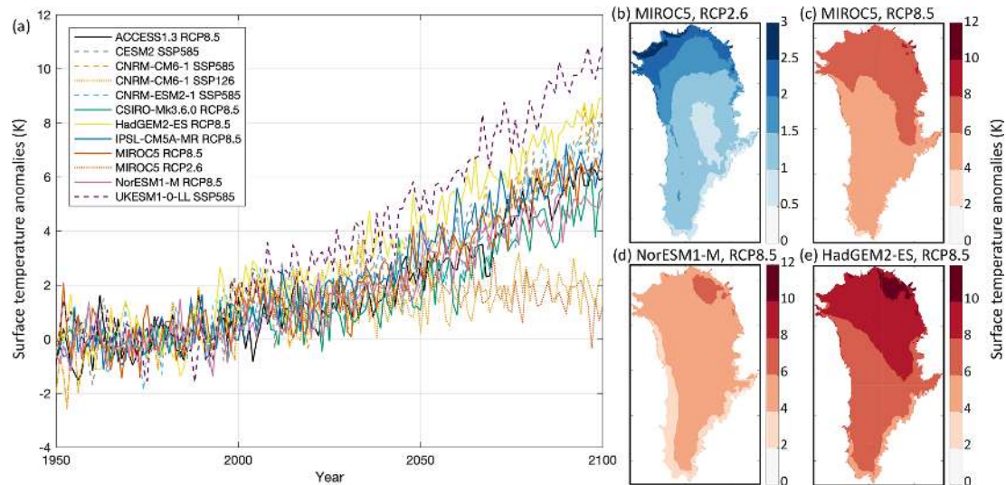
Figure 4. Surface temperature anomalies (K) over the Greenland ice sheet under the RCP2.6, RCP8.5, SSP1-2.6, and SSP5-8.5 scenarios. (a) Time series of mean surface temperature anomaly from 1950 to 2100 for all AOGCMs and scenarios selected and (b–e) surface temperature anomaly over the time period 2081–2100 for (b) MIROC5 under RCP2.6, (c) MIROC5 under RCP8.5, (d) NorESM1-M under RCP8.5, and (e) HadGEM2-ES under RCP8.5.
