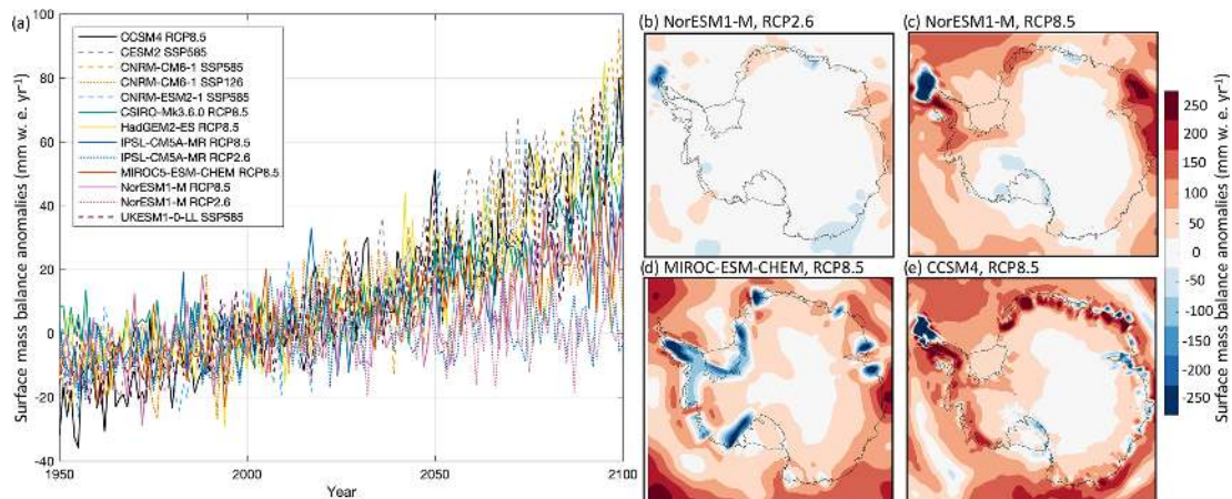
Figure 3. Surface mass balance anomalies ( \text{mm w.e. yr}^{-1} ) over the Antarctic ice sheet under the RCP2.6, RCP8.5, SSP1-2.6, and SSP5-8.5 scenarios. (a) Time series of mean surface mass balance anomaly from 1950 to 2100 for all AOGCMs and scenarios selected and (b–e) mean surface mass balance anomaly over the time period 2081–2100 for (b) NorESM1-M under RCP2.6, (c) NorESM1-M under RCP8.5, (d) MIROC-ESM-CHEM under RCP8.5, and (e) CCSM4 under RCP8.5.
