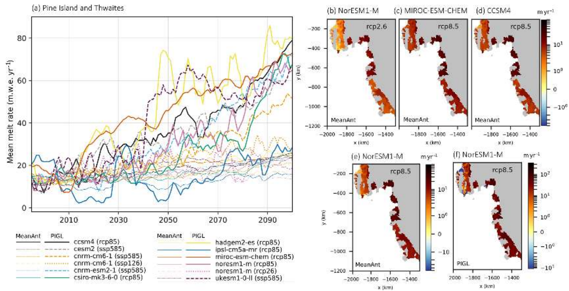
Figure 7. Mean cavity basal melt rates ( \text{m w.e. yr}^{-1} ) under the RCP2.6, RCP8.5, SSP1-2.6, and SSP5-8.5 scenarios over the 21st century for MeanAnt and PIGL calibrations and nonlocal parameterizations in the Amundsen Sea sector. (a) Time series for Pine Island and Thwaites ice shelves obtained with MeanAnt (thin lines) and PIGL (thick lines) calibrations (adapted from Jourdain et al., 2020). Spatial patterns of mean sub-shelf basal melt rate from 2081 to 2100 for the Tier 1 models assuming MeanAnt calibration for (b) NorESM1-M under RCP2.6, (c) MIROC-ESM-CHEM under RCP8.5, (d) CCSM4 under RCP8.5, and (e) NorESM1-M under RCP8.5 and PIGL calibration for (f) NorESM1-M under RCP8.5. The projections from the MeanAnt and PIGL calibrations assume that the ice shelf cavities have not evolved and are set to the present day.
