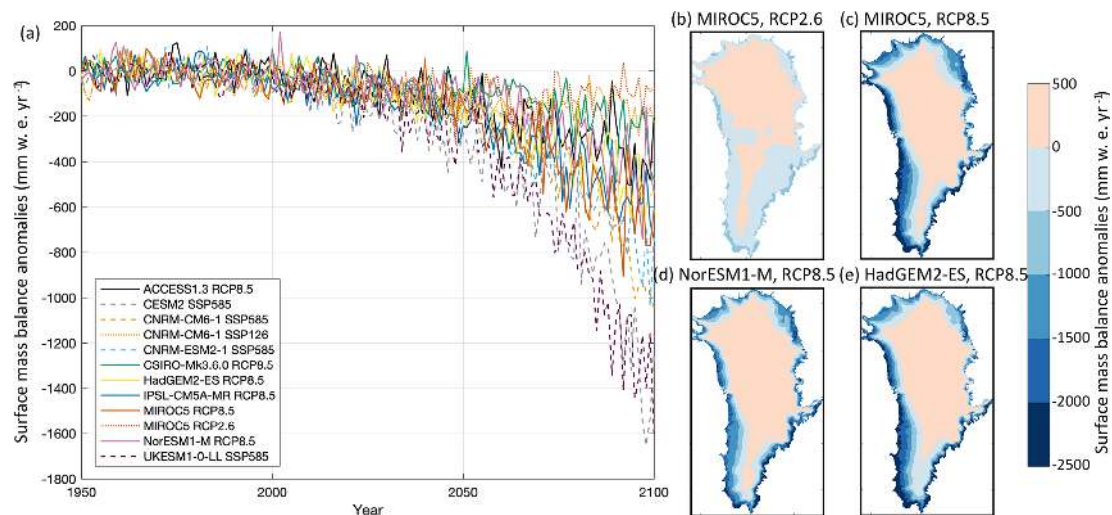
Figure 5. Surface mass balance anomalies ( \text{mm w. e. yr}^{-1} ) over the Greenland ice sheet under the RCP2.6, RCP8.5, SSP1-2.6, and SSP5-8.5 scenarios. (a) Time series of mean surface mass balance anomaly from 1950 to 2100 for all AOGCMs and scenarios selected and (b–e) mean surface mass balance anomaly over the time period 2081–2100 for (b) MIROC5 under RCP2.6, (c) MIROC5 under RCP8.5, (d) NorESM1-M under RCP8.5, and (e) HadGEM2-ES under RCP8.5.
