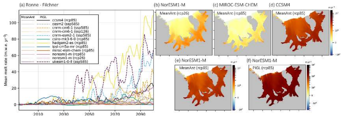
Figure 8. Mean cavity basal melt rates ( \text{m w.e. yr}^{-1} ) under the RCP2.6, RCP8.5, SSP1-2.6, and SSP5-8.5 scenarios over the 21st century for MeanAnt and PIGL calibrations and nonlocal parameterizations in the Weddell Sea sector. (a) Time series for the Ronne–Filchner ice shelf obtained with MeanAnt (thin lines) and PIGL (thick lines) calibrations (adapted from Jourdain et al., 2020). Spatial patterns of mean sub-shelf basal melt rate from 2081 to 2100 for the Tier 1 models assuming MeanAnt calibration for (b) NorESM1-M under RCP2.6, (c) MIROC-ESM-CHEM under RCP8.5, (d) CCSM4 under RCP8.5, and (e) NorESM1-M under RCP8.5 and PIGL calibration for (f) NorESM1-M under RCP8.5. The projections from the MeanAnt and PIGL calibrations assume that the ice shelf cavities have not evolved and are set to the present day.
