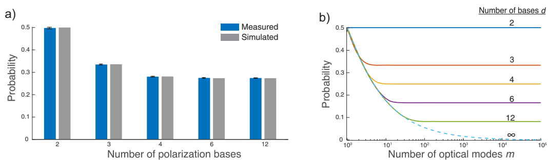
Fig. 4 Privacy of the input state for the computation. A nearly optimal attack is for Bob to measure all of Alice’s photons in a randomly chosen basis. The security of Alice’s input depends on the number d of polarization bases (keys) d she can choose from and also the number of input modes m . a Probability of Bob correctly guessing Alice’s input for m=4 , as key size is increased from d=2 to d=12 . b Calculated probability of correctly guessing the input with respect to number of bases d (lines) and modes m . The blue dashed line shows the asymptotic behavior for an infinite key number. All lines are theoretical upper bounds (see “Methods” for formula).
