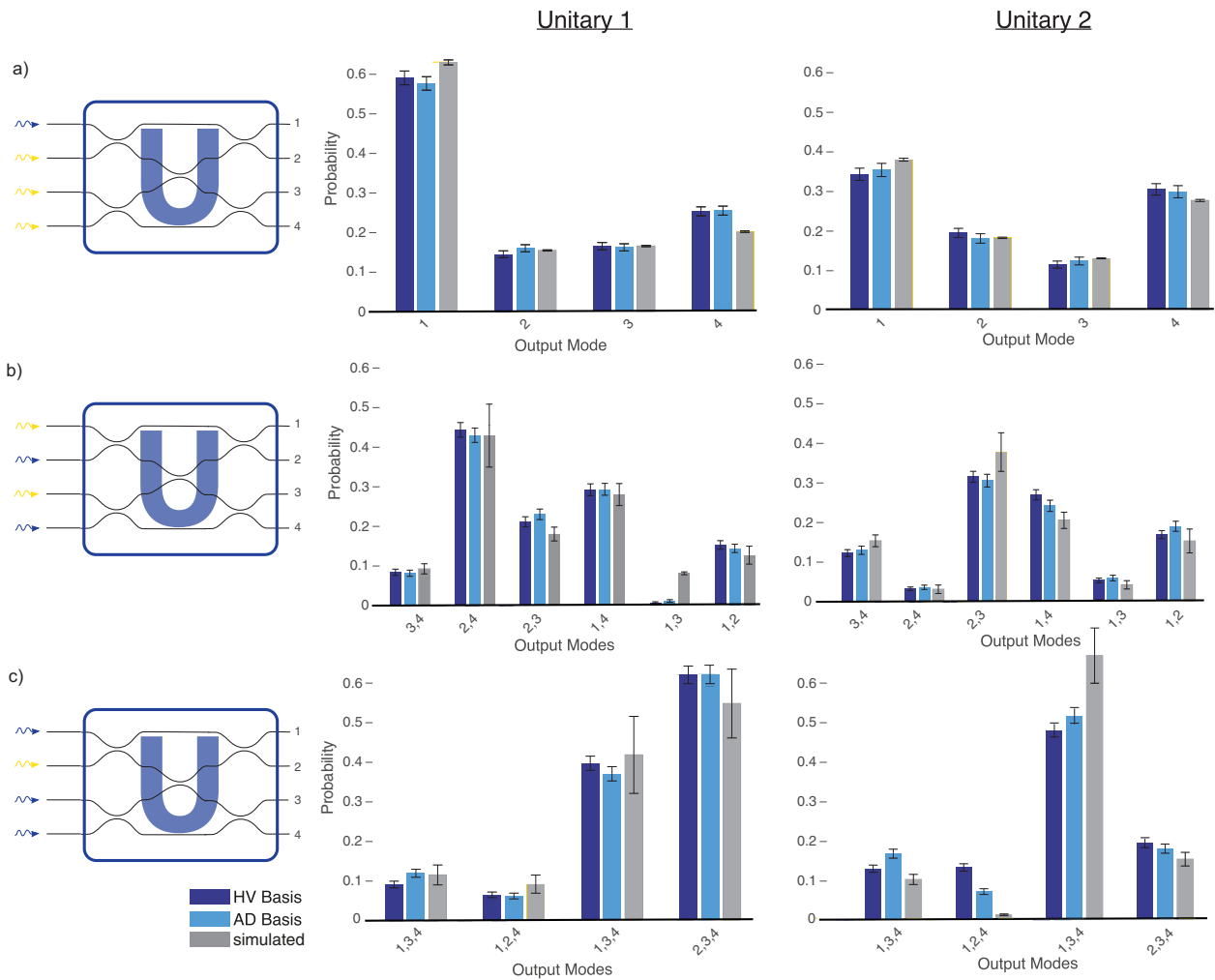
Fig. 3 Results of the encrypted quantum walk. We use two different unitaries to execute multiple encrypted quantum walk computations. a Unitary transformation of a single-photon state, b quantum walk with two photons, and c quantum walk with three photons. Blue photons represent data photons, whereas yellow photons are ancilla photons used to mask the computation that is performed (see Fig. 1). The output probability distribution for two different unitaries is shown. In each case, the computation was performed in two mutually unbiased polarization bases (see “Supplementary Information”). The fidelities (Bhattacharyya distance 18 ) between the simulated (see “Methods”) and measured probabilities are a 0.99 \pm 0.02 , b 0.99 \pm 0.02 , and c 0.99 \pm 0.03 and demonstrate the polarization independence of the computation. More data and discussion of error analysis is provided in “Methods” and the “Supplementary Information”.
