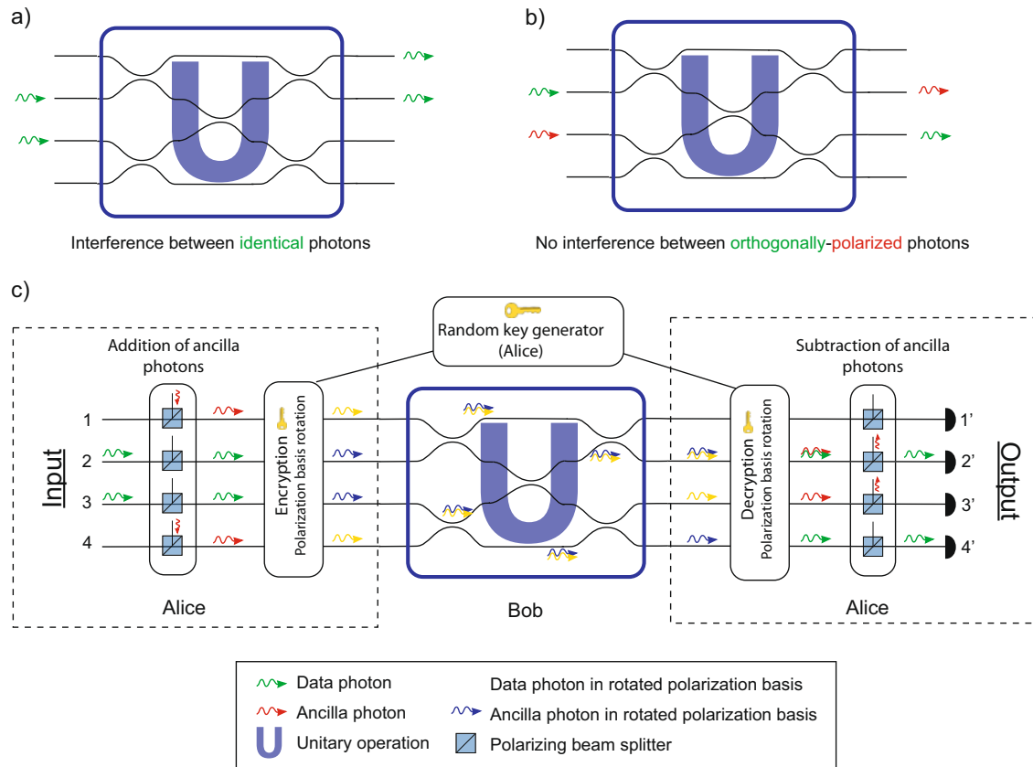
Fig. 1 Homomorphic encryption scheme. a Phase shifters and directional couplers can be used to implement any desired unitary transformation for arbitrary dimensions, either for single- or multi-photon states 27,28 . In the case of indistinguishable photons entering the circuit simultaneously, quantum interference leads to nontrivial outputs of a so-called quantum walk computation. b If two orthogonally polarized photons enter the circuit at the same time they are distinguishable and therefore no quantum interference takes place. c In the implemented quantum homomorphic encryption scheme, Alice prepares her input state by encoding the desired photon-number state in the \{|H\rangle, |V\rangle\} polarization basis and then encrypting it by applying a randomly chosen polarization transformation on all photons. Bob performs the quantum computation on the encrypted state and returns the photons to Alice. Alice undoes the previous transformation ( R^{-1} ) and measures the photons in the \{|H\rangle, |V\rangle\} basis, obtaining the outcome of the quantum computation. Since Bob has no information about the polarization basis chosen by Alice, his information about Alice's input state is limited.
