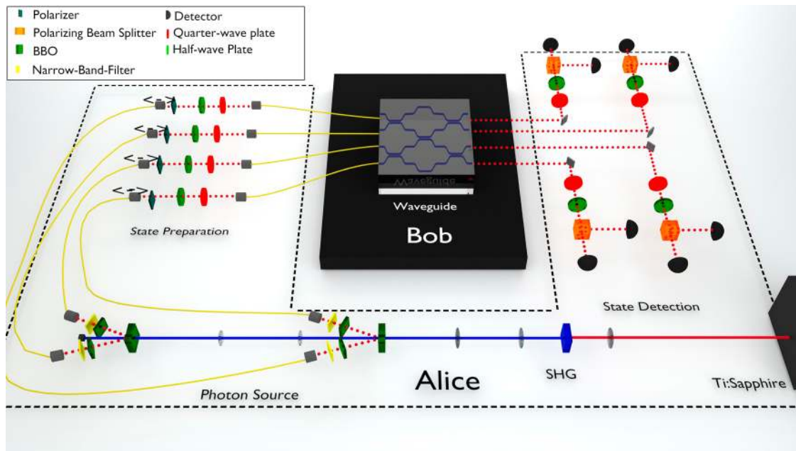
Fig. 2 Experimental setup. A Ti:Sapphire laser is used to pump two nonlinear \beta -barium borate crystals, each probabilistically producing exactly one pair via type-II spontaneous parametric down conversion. These photons are spectrally filtered and sent through polarizers to prepare a pure, separable four-photon state. The four photons are coupled to single-mode fibers and synchronized in the delay stage, using adjustable free-space delays (indicated by the double arrows). Using half-wave plates (HWPs) and quarter-wave plates (QWPs) Alice can prepare arbitrary polarization states before sending the photons to Bob, who will perform the quantum walk. After exiting Bob's chip, the four output modes are collimated by a lens and sent back to Alice. She uses the detection stage (HWP, QWP, polarizing beam splitter (PBS), and single-photon detector for each photon) to projectively measure the photons and recover the outcome of the quantum walk.
