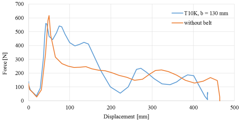
Fig. 6. Characteristics of the change in cutting force of the strong flexible belts
