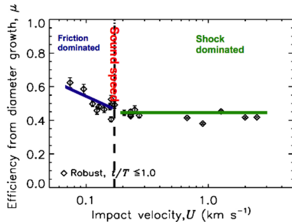
Figure 3: Preliminary results showing changes in the efficiency parameter \mu = 1/(\text{rate of crater growth}) with impact velocity.
