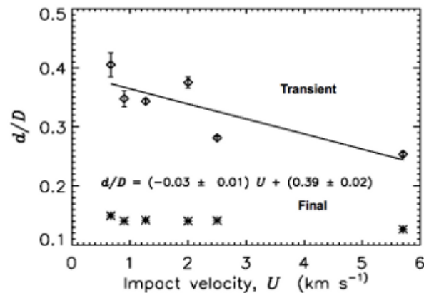
Figure 4: Preliminary results showing changes in the transient and final diameter-to-depth ratio of craters with impact velocity.
