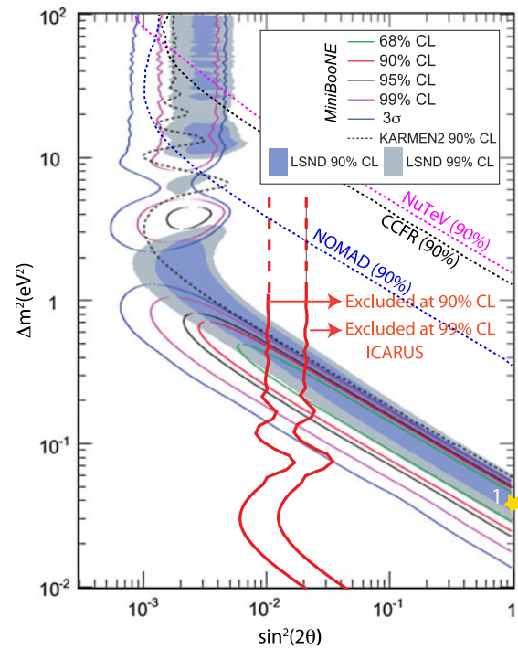
Fig. 5 Two-dimensional plot of \Delta m^2 vs \sin^2(2\theta_{\text{new}}) for the main published experiments sensitive to the \nu_\mu \rightarrow \nu_e anomaly [2, 3, 31–34] and the present ICARUS result. The ICARUS limits to the oscillation probability are \langle P_{\nu_\mu \rightarrow \nu_e} \rangle \leq 5.4 \times 10^{-3} and \langle P_{\nu_\mu \rightarrow \nu_e} \rangle \leq 1.1 \times 10^{-2} , corresponding to \sin^2(2\theta_{\text{new}}) \leq 1.1 \times 10^{-2} and \sin^2(2\theta_{\text{new}}) \leq 2.2 \times 10^{-2} respectively at 90 % and 99 % CL. Limits correspond to 3.41 and to 7.13 events
