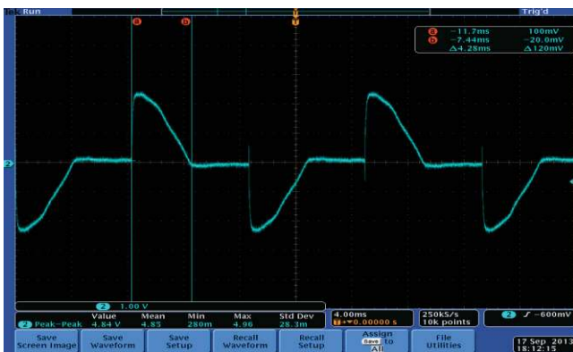
Figure 12: Plot of voltage across the terminals of the CFL with dimmer level set to 50.
