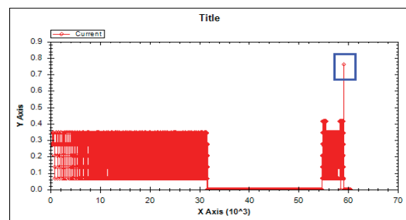
Figure 15: Resultant spike from current surge in CFL.
