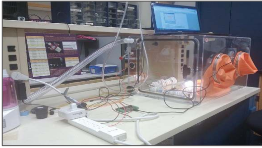
Figure 3: Glove box used to contain shattered glass and mercury.
