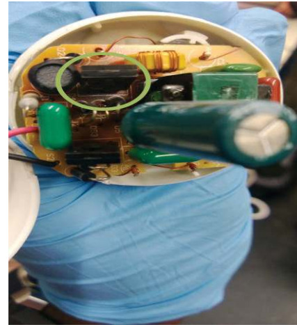
Figure 14: Charred CFL.
