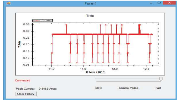
Figure 6: Real-time Plotting Utility Reporting Current Consumption.
