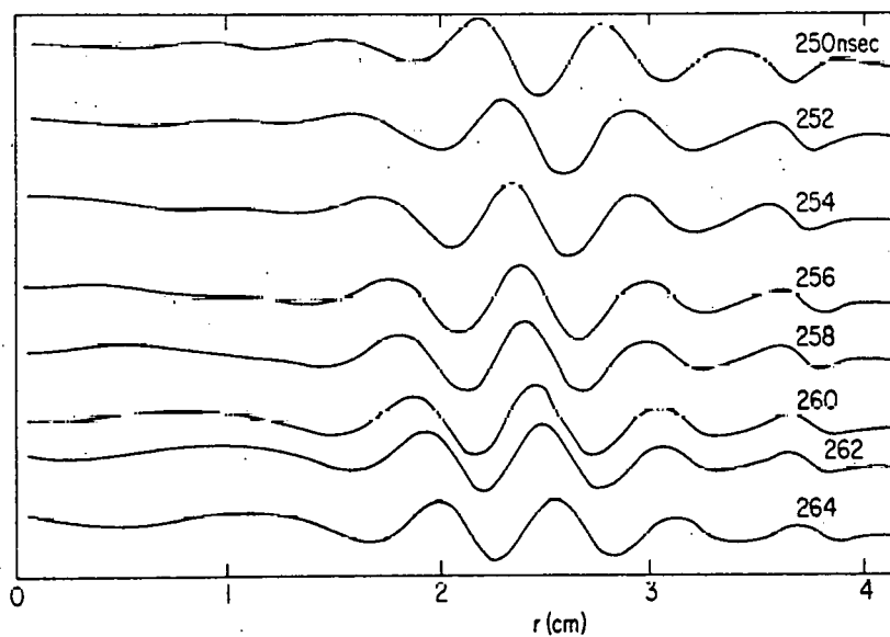
Fig. 12. Radial motion of the wave phase using the boxcar integrator circuit, same settings as Fig. 11 except that the time between successive traces is now much less a wave period. The wave phase moves radially out of the plasma with increased time.
