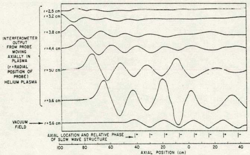
Fig. 4. Axial probe interferometer signal. The axial traces made at different radial positions show the conical trajectory of the wave. The bottom trace is the vacuum field of the slow wave structure.
