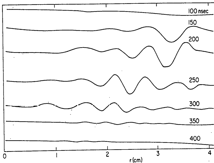
Fig. 11. Radial motion of wave packet using the boxcar integrator circuit. The wave packet moves radially into the plasma with increased time. f=40 MHz.
