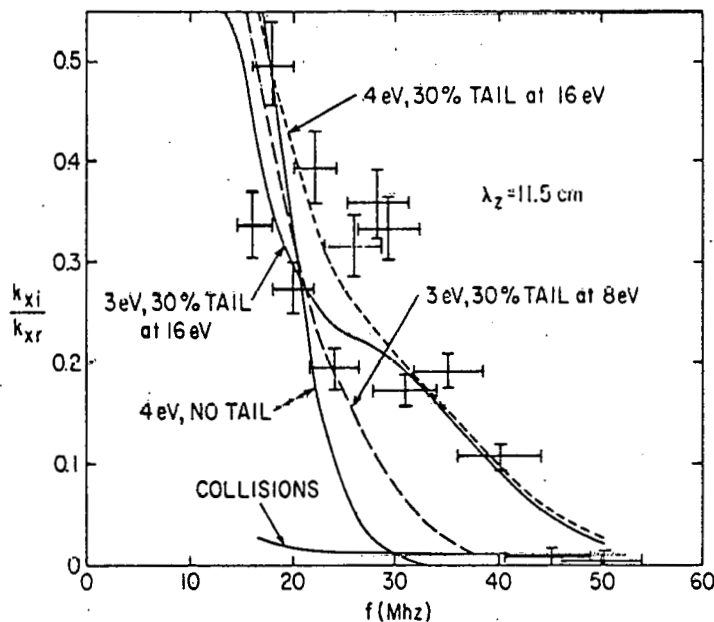
Fig. 16. Damping ratio k_{xi}/k_{xr} for the high pressure ( p \sim 3\mu ) equilibrium; He, B=1.3 kG, \lambda_z=11.5 cm. The experimental measurements (|—|) are in reasonable agreement with the Landau damping from an electron distribution function consisting of a 4 eV main body and a \sim 30\% , 16 eV tail. Again, the experimentally observed damping is too large to be explained by collisional damping or main body Landau damping.
