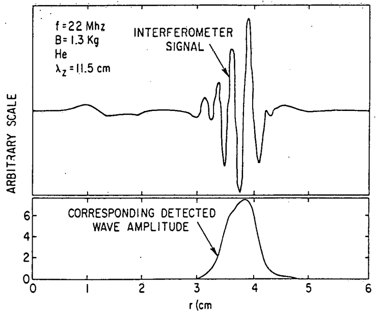
Fig. 14. Bottom: Typical amplitude signal measured using a doubled tipped rf probe as described in Section IV (high pressure equilibrium; \lambda_z = 11.5 cm). Top: Interferometer trace of the same signal.
