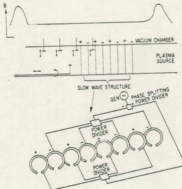
Fig. 2. Experimental setup. The eight rings driven by power dividers alternate in phase by 180^\circ .
