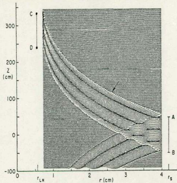
Fig. 1. Plots of field generated by a 100 cm long slow wave structure (located along the line AB). \lambda_z = 33.3 cm; density profile is Lorentzian, n(r) = 10^{12} [1 + (r/0.75)^2] ; f=50 MHz; B=2 Kg; He gas. Sharp logarithmic singularities shown as blanks (arrow) bound the wave field.
