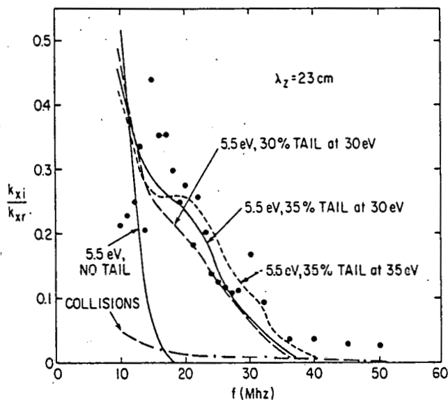
Fig. 15. Damping ratio k_{xi}/k_{xr} for the low pressure ( p \sim 0.5\mu ) equilibrium, He, B=1.3 kG, \lambda_z=23 cm. The experimental measurements (dots) are in reasonable agreement with Landau damping from an electron distribution function consisting of a 5.5 eV main body and a \sim 30\% , 30 eV tail. The experimentally observed damping is too large to be explained by collisional damping or solely main body Landau damping.
