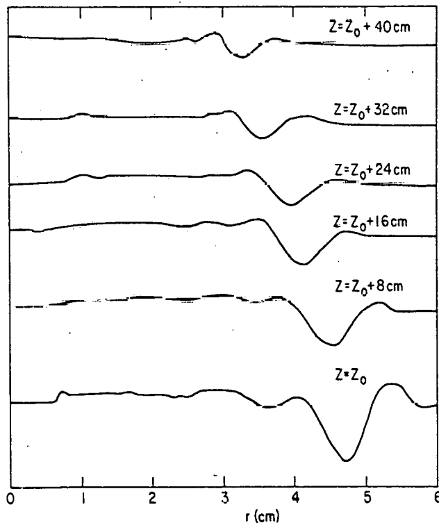
Fig. 8. Interferometer signal for a sequence of axial positions at 12 MHz (the plasma conditions are identical with those of Figs. 6 and 7). The wave packet is radially further out than the 20 MHz case and appears to be more strongly damped. However, this interferometrically observed damping comes from phase decorrelation (c.f. Fig. 9 and discussion in text).
