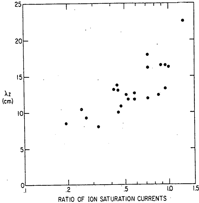
Fig. 5. \lambda_z vs. the ratio of the ion saturation currents from two probes separated axially by 150 cm. When the density gradient is weak, the probe currents are approximately the same, and \lambda_z corresponds to the wavelength imposed by the slow wave structure. When the density gradient is large, \lambda_z becomes shorter, in qualitative agreement with Eq. (1). These measurements were obtained by varying the filling pressure and/or the mirror field.
