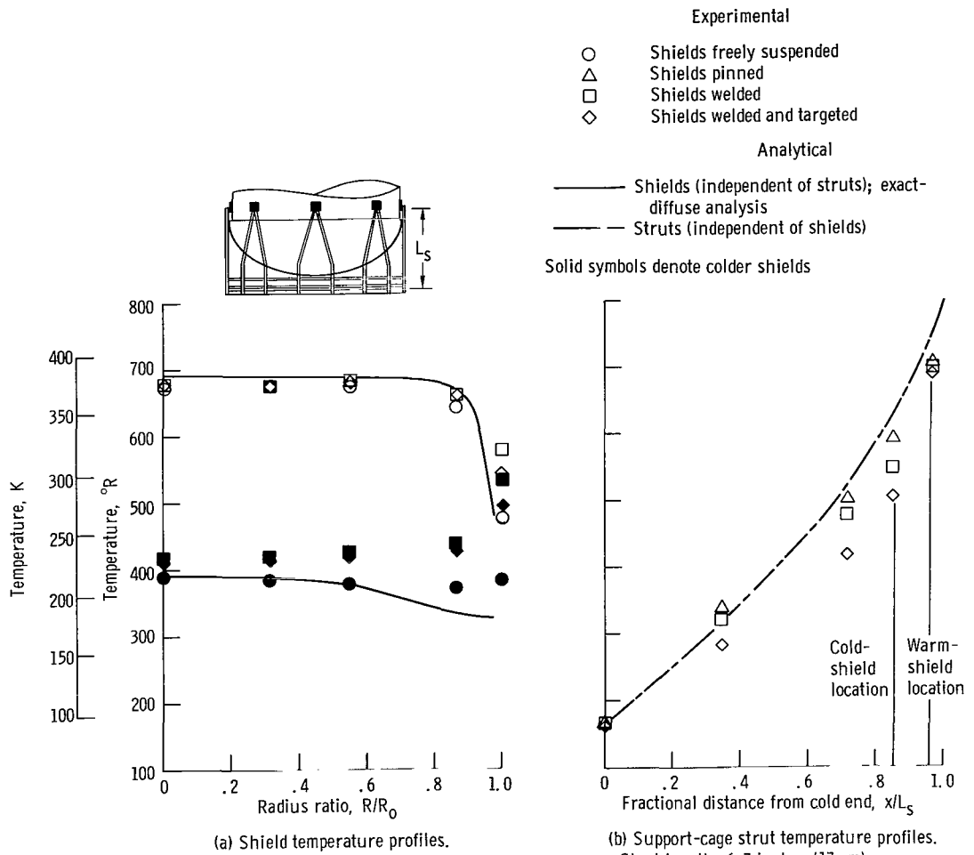
Figure 32. - Shield and support-cage temperature profiles for pinned, welded, and targeted systems (shield IX). L/R_0 = 0.192 .
