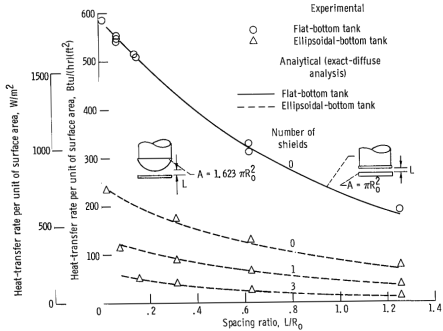
Figure 27. - Effect of tank shape on heat-transfer rate for several configurations (shield I). Surface area of ellipsoidal bottom is 1.623 times surface area of flat bottom. Heater temperature, 800° R (444 K); tank temperature, 140° R (77.8 K).
