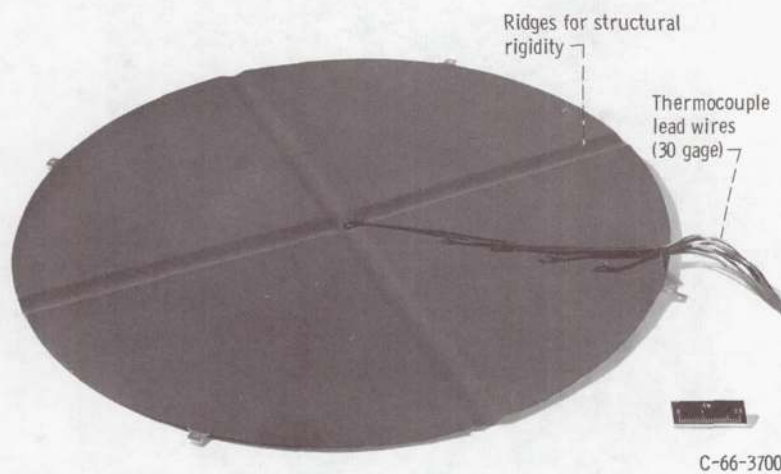
Figure 4. - Construction method for 0.015-inch (0.0381-cm) stainless-steel shield (shield V).
