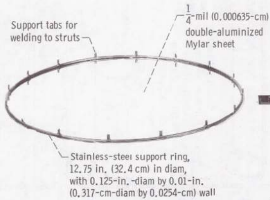
Figure 6. - Single-sheeted shield with support tabs (representative of shield IX).
