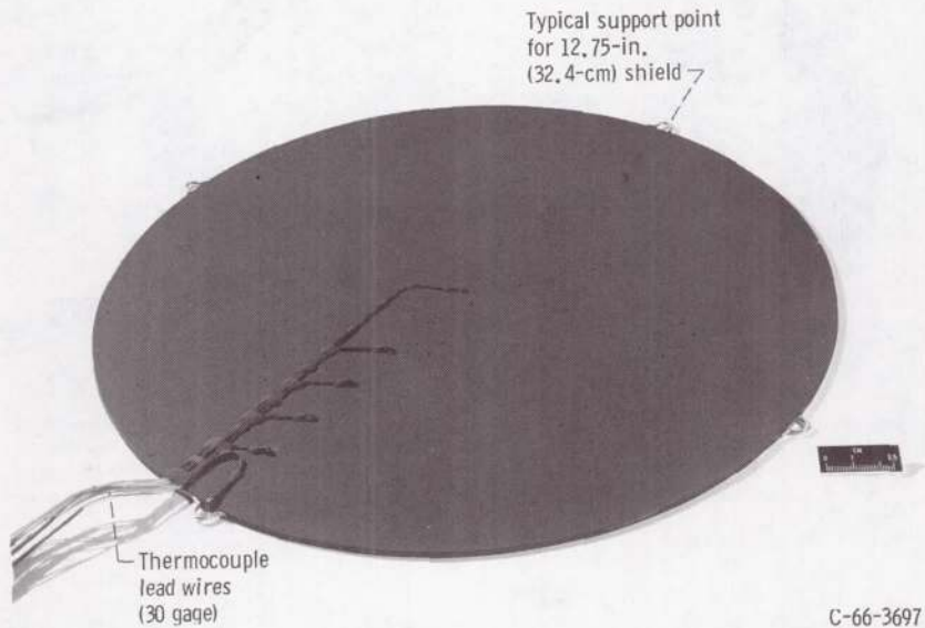
Figure 3. - Typical construction and instrumentation used for relatively thick copper, stainless-steel, and aluminum shadow shields (shields I, II, III, and IV).
