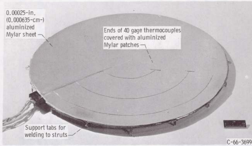
Figure 10. - Double-sheeted shield with structural support welding tabs.
