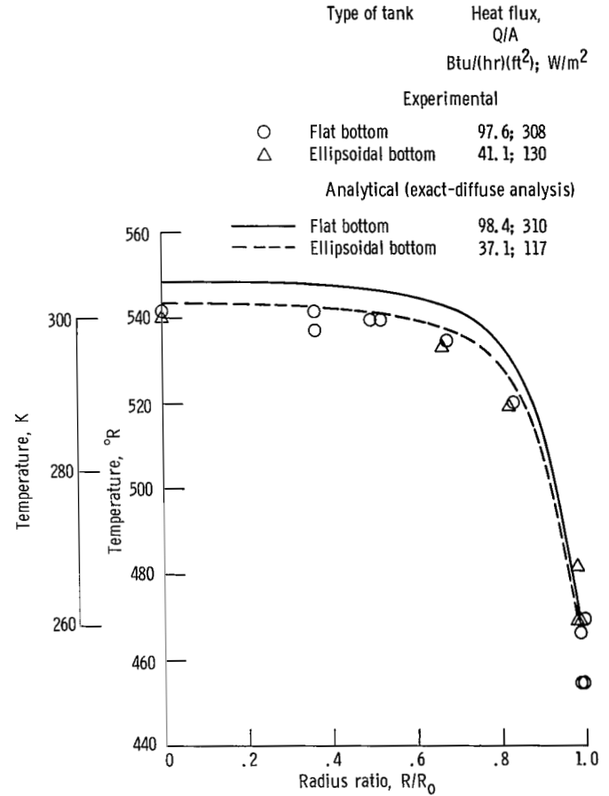
Figure 28. - Effect of tank shape on temperature profile of a single low-conducting shield (shield VI). Heater temperature, 650° R (361 K); spacing ratio, 0.314.
