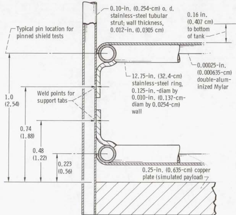
Figure 9. - Shield construction and method of mounting for integrated shadow shield system. (Dimensions are in inches (cm).)
