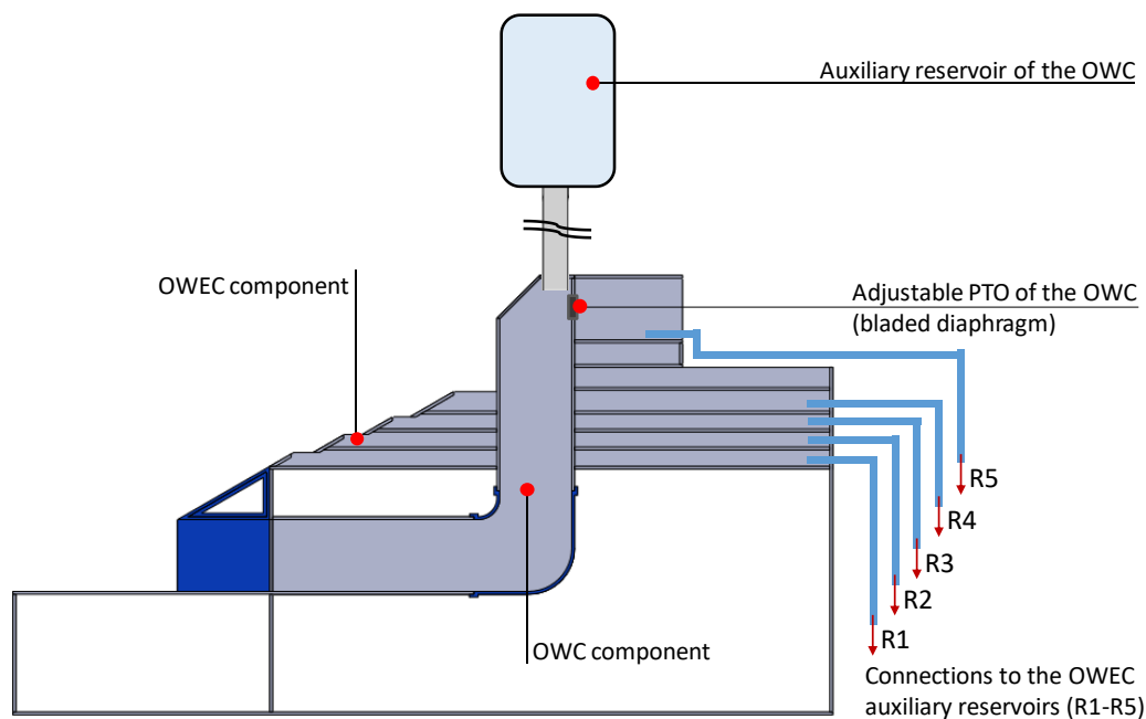
Figure 6. Hybrid WEC module: schematic representation of the cross-section.
