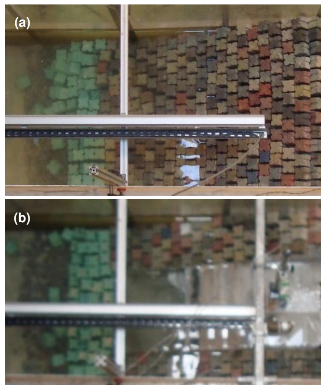
Figure 12. Rubble-mound breakwater after the conclusion of the tests of TS1 (a) and TS3 (b).
