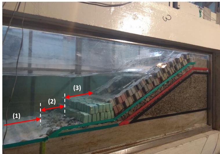
Figure 11. Physical model of the breakwater with the hybrid WEC module integrated: (1) sandy sea bottom, (2) rubble foundation, and (3) toe berm of the breakwater.
