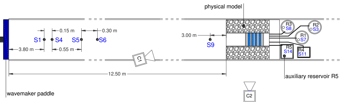
Figure 4. Physical model setup in the channel built inside the wave basin of FEUP.
