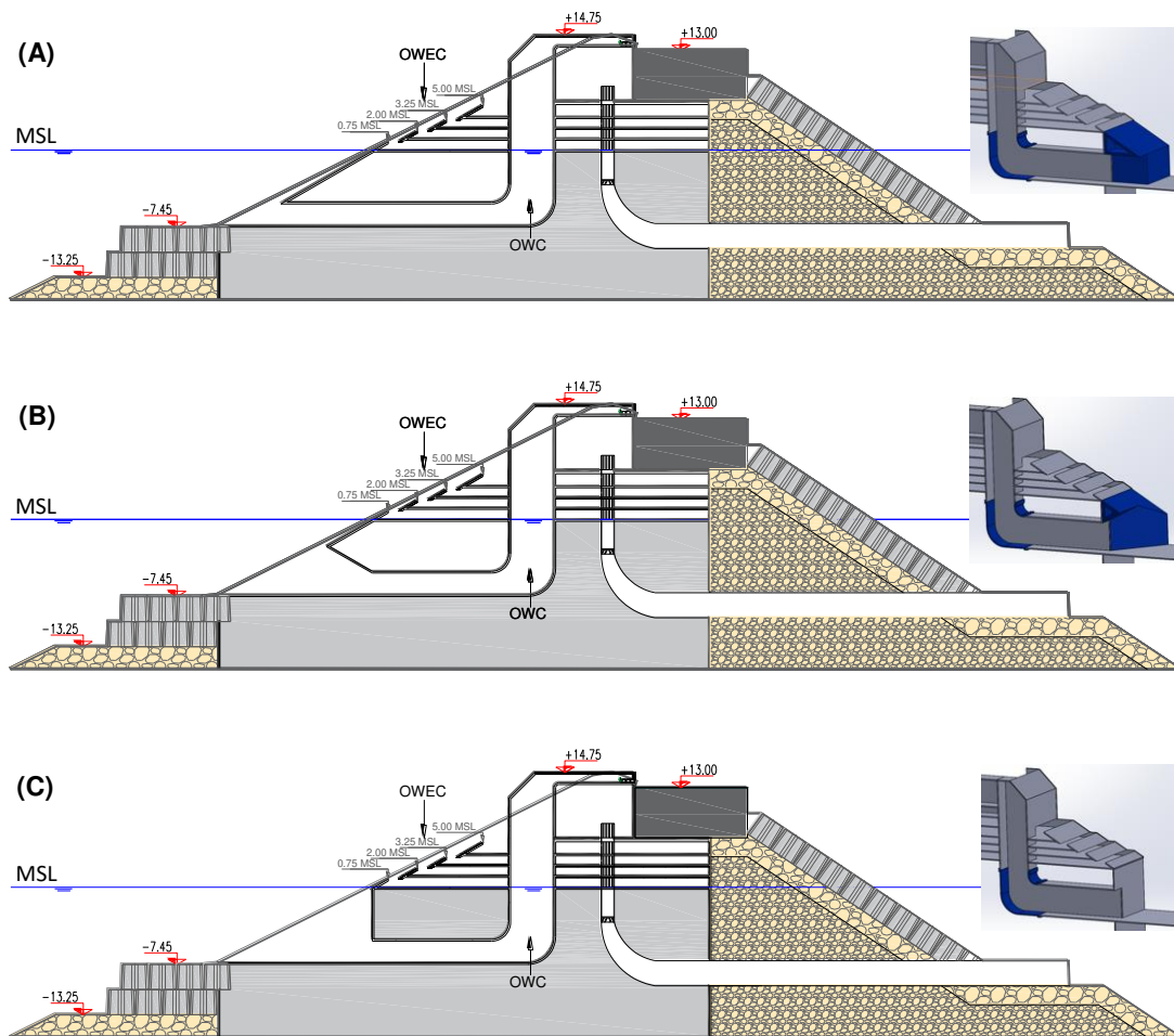
Figure 7. Geometries A, B, and C of the hybrid WEC tested (full-scale dimensions) and detail of OWC intake.
