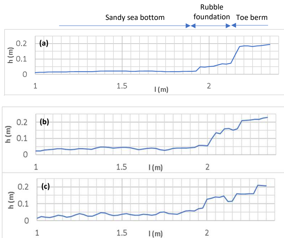
Figure 10. Variation of the bathymetry in front of the breakwater toe: initial bathymetric profile (a) and profiles after test series TS1 (b) and TS3 (c).
