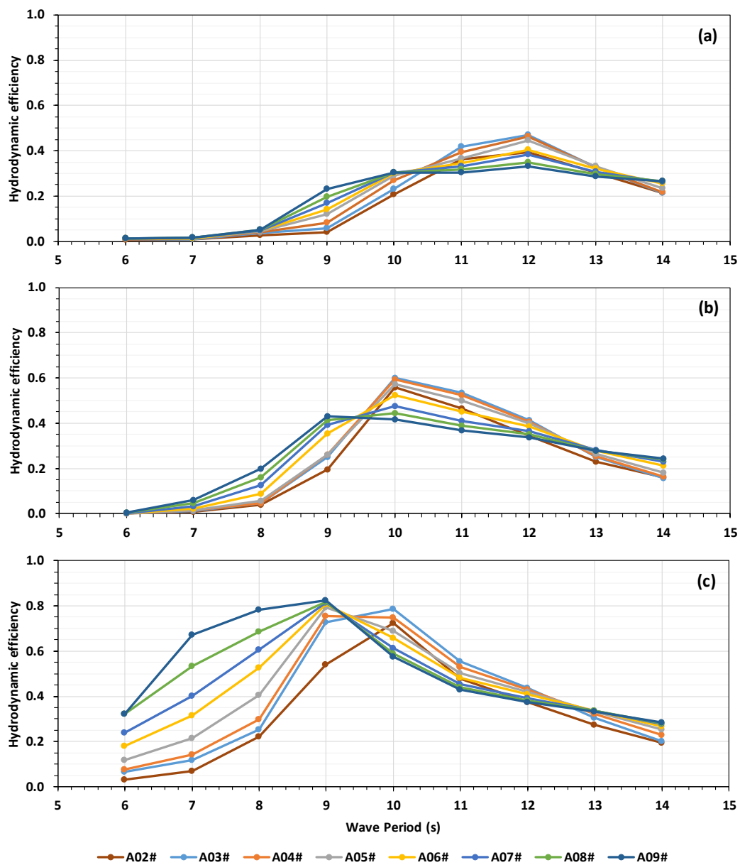
Figure 9. Efficiency of the OWC for the three tested geometries considering the different PTO damping values: (a) geometry A, (b) geometry B, and (c) geometry C.
