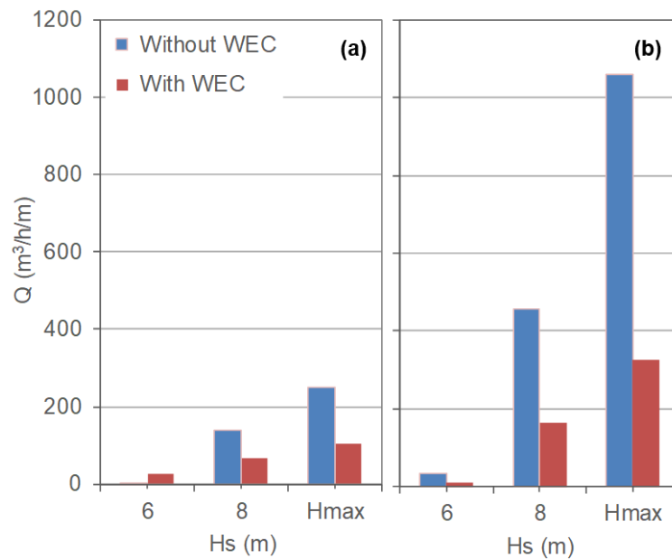
Figure 13. Mean overtopping flow rates obtained for TS1 and TS3, and for the two water levels: low tide—MLWS (a) and high tide—MHWS (b).
