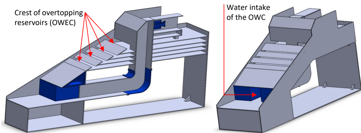
Figure 5. 3D sketch of the hybrid wave energy converter.
