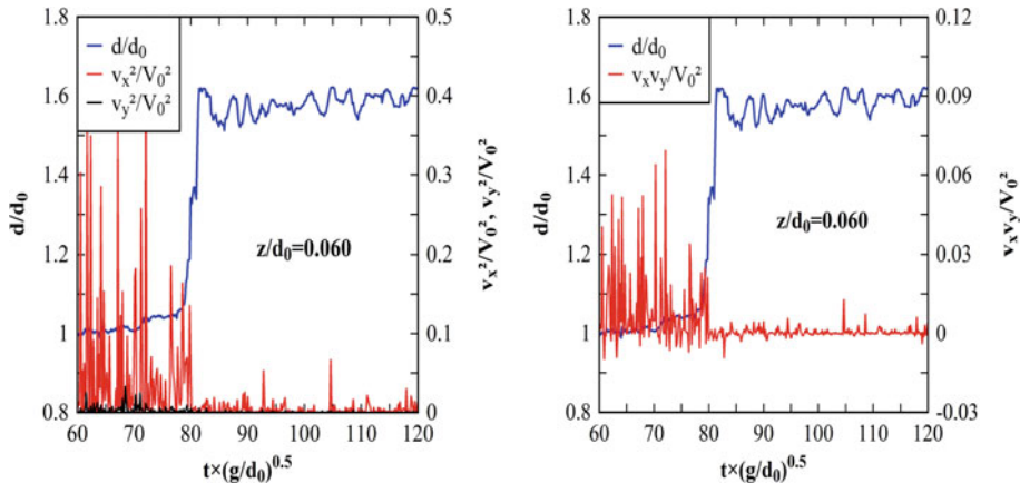
Fig. 9 Breaking surge, Run 60-6. Dimensionless instantaneous water depth d/d_0 and normal Reynolds stresses v_x^2/V_0^2 and v_y^2/V_0^2 (left) and tangential Reynolds stresses v_x v_y/V_0^2 (right) at z/d_0 = 0.060
