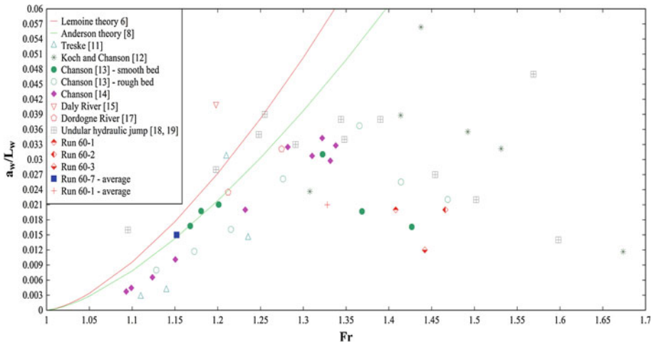
Fig. 3 Dimensionless characteristics of undular bores. Wave steepness
