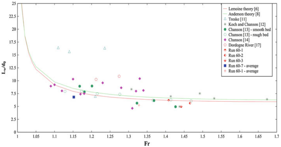
Fig. 2 Dimensionless characteristics of undular bores. Wave length
