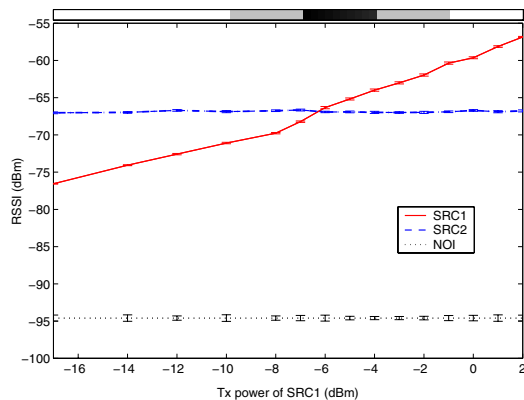
(b) Transmission power level to RSS
