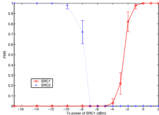
(a) Transmission power level to PRR
