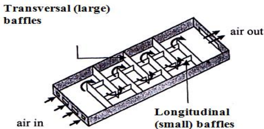
Figure 7: Solar panel equipped with TL type baffles [Kg/KgMS: kilograms of water per kilograms of dried mass of the product]
