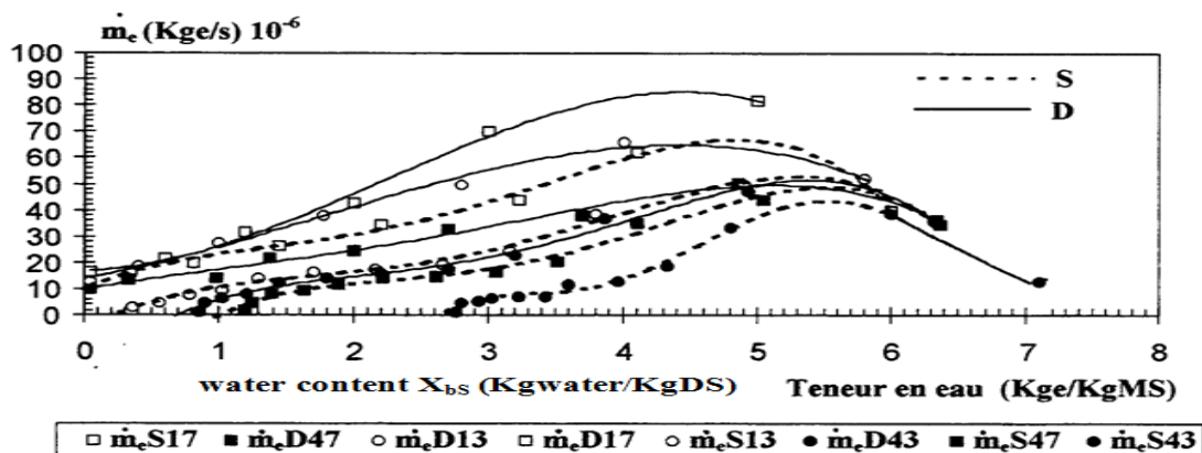
Figure 11: Evolution of the drying speed ( m_e ) in relation to water content to the point when the product is completely dried with flows of 31.3\text{m}^3/\text{h.m}^2 and 70\text{m}^3/\text{h.m}^2 using WB and DCL1 type solar panels
