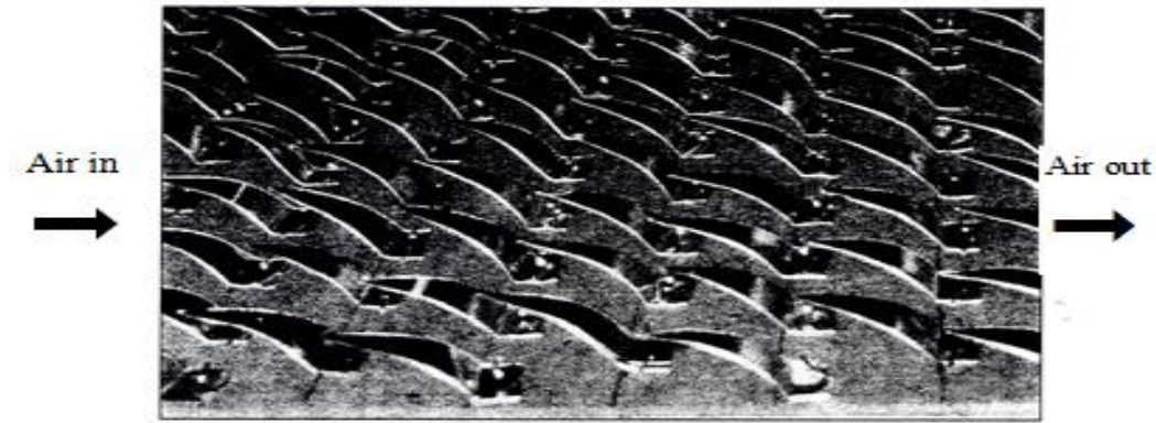
Photograph 2: Layout with OCL1 type baffles
