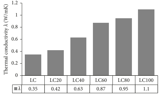
FIGURE 8: Effect of SWM dosage on the thermal conductivity of LC at 28 days.
