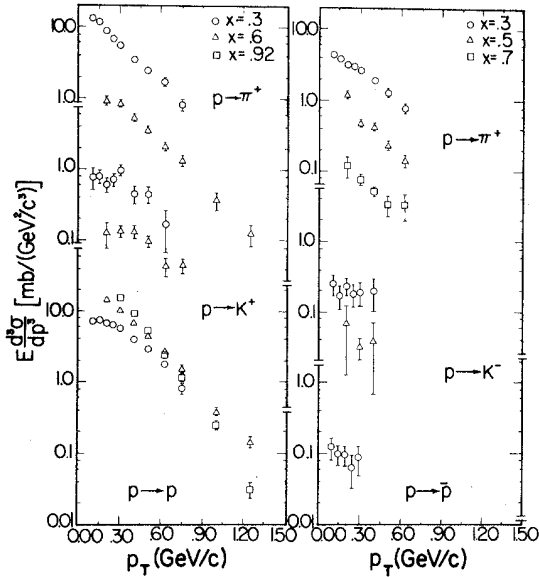
FIG. 17. The invariant differential cross section for proton-induced reactions is shown as a function of transverse momentum p_T . The incident energy is 100 GeV.
