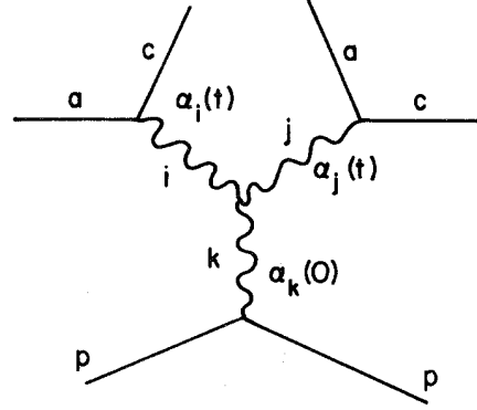
FIG. 20. Triple-Regge-exchange diagram for the process a + p \rightarrow c + X for s/M_X^2 \gg 1 and s \rightarrow \infty .
