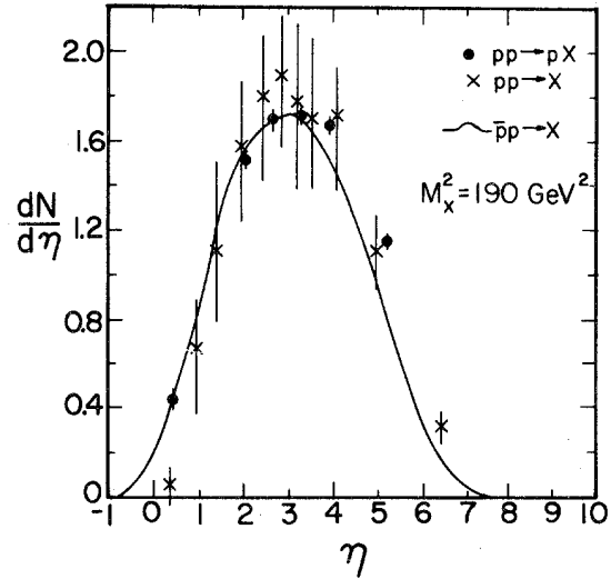
FIG. 30. Pseudorapidity distribution for associated particles in pp \rightarrow pX compared with pseudorapidities for pp \rightarrow X (Ref. 47), and \bar{p}p \rightarrow X (Ref. 48) at a common s = M_X^2 = 190 \text{ GeV}^2 .
