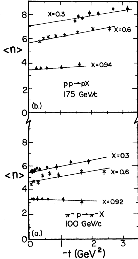
FIG. 26. Dependence of the associated-charged-particle multiplicity for pp \rightarrow pX and \pi^- p \rightarrow \pi^- X on the invariant momentum transfer t at fixed x . Linear-fit parameters are displayed in Figs. 28 and 29.
