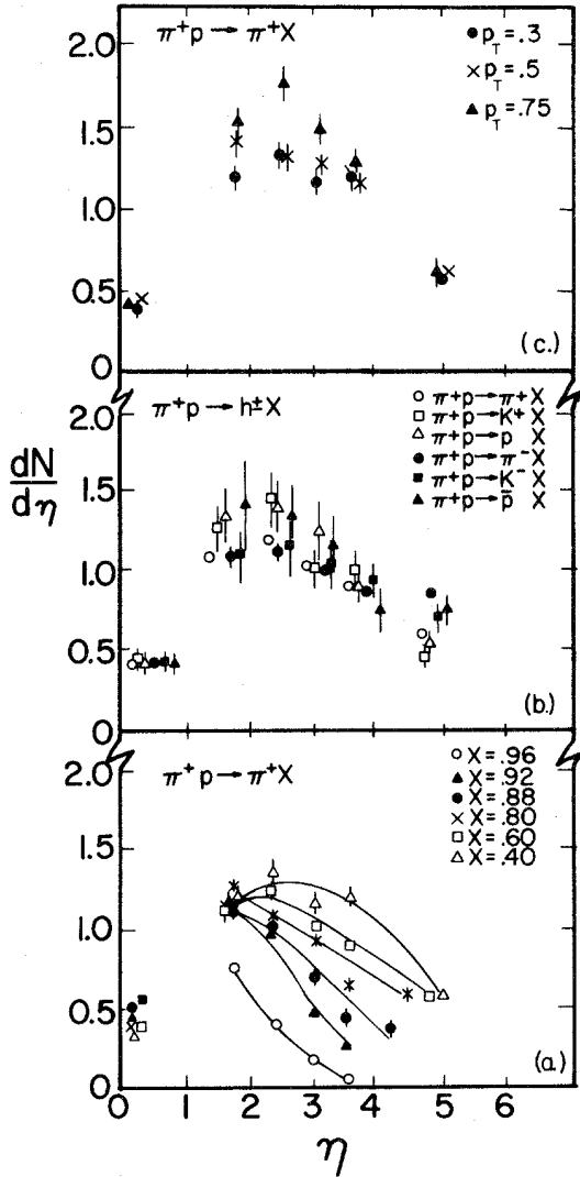
FIG. 31. Pseudorapidity distributions. (a) x dependence for \pi^+ p \rightarrow \pi^+ X at p_T = 0.3 GeV/c. Curves are drawn to guide the eye. (b) Trigger-particle dependence for \pi^+ p \rightarrow h^\pm X for 100-GeV/c incident \pi^+ at x = 0.6 and p_T = 0.3 GeV/c. (c) p_T dependence for \pi^+ p \rightarrow \pi^+ X at x = 0.4 for 100-GeV/c \pi^+ .
