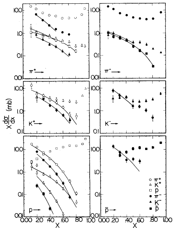
FIG. 19. The integrated cross section x d\sigma/dx as a function of x for incident energy of 175 GeV.
