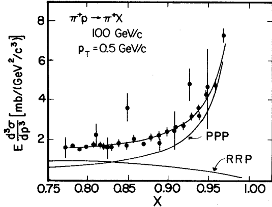
FIG. 22. Fine-binned data for \pi^+p \rightarrow \pi^+X at 100 GeV/c and p_T = 0.5 GeV/c with PPP and RRP contributions to the triple-Regge fit.
