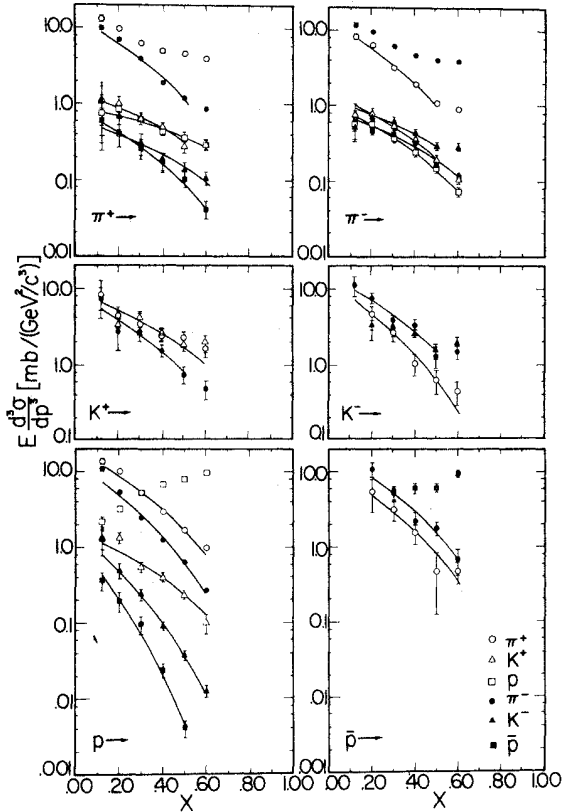
FIG. 13. The invariant differential cross section is shown as a function of x , for an incident energy of 175 GeV and a transverse momentum p_T of 0.3 GeV/c. There is one subfigure for each incident-particle type. Comparisons to a functional form C(1-x)^n are shown.
