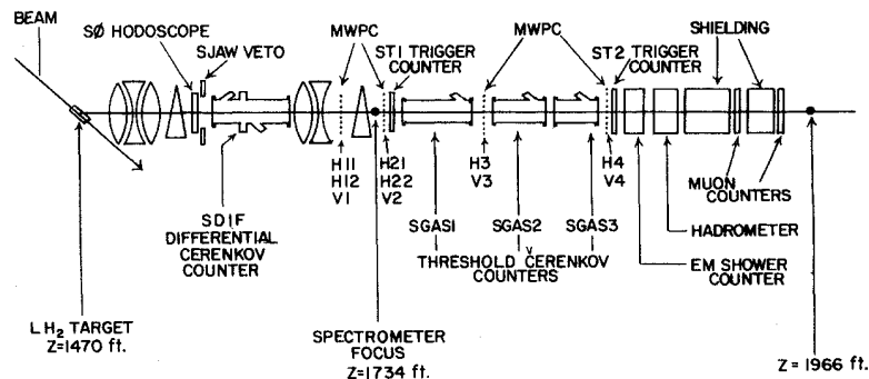
FIG. 4. The Single Arm Spectrometer instrumentation. The quadrupole polarities are indicated for the nonbend, vertical plane.
