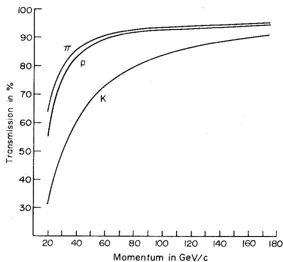
FIG. 7. The spectrometer transmission for \pi , K , and protons as a function of spectrometer momentum. These curves include the effects of nuclear and multiple scattering as well as decays.
