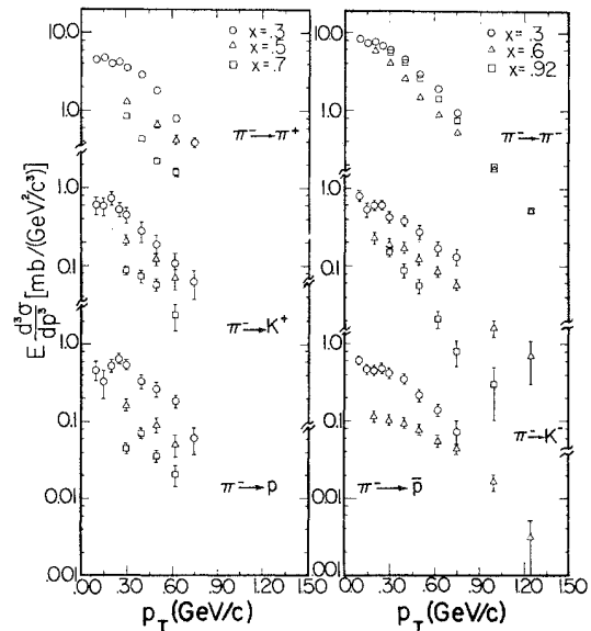
FIG. 16. The invariant differential cross section for \pi^- -induced reactions is shown as a function of transverse momentum p_T . The incident energy is 100 GeV.
