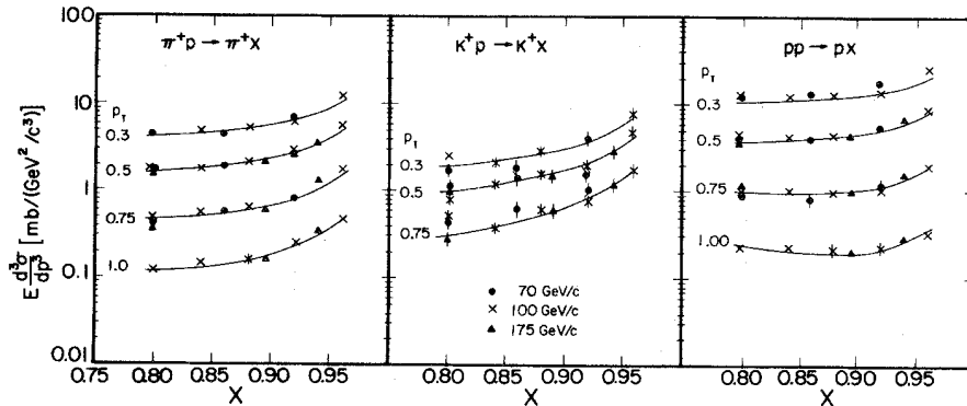
FIG. 21. Data and triple-Regge fits to \pi^+p \rightarrow \pi^+X , K^+p \rightarrow K^+X , and pp \rightarrow pX at 70, 100, and 175 GeV.
