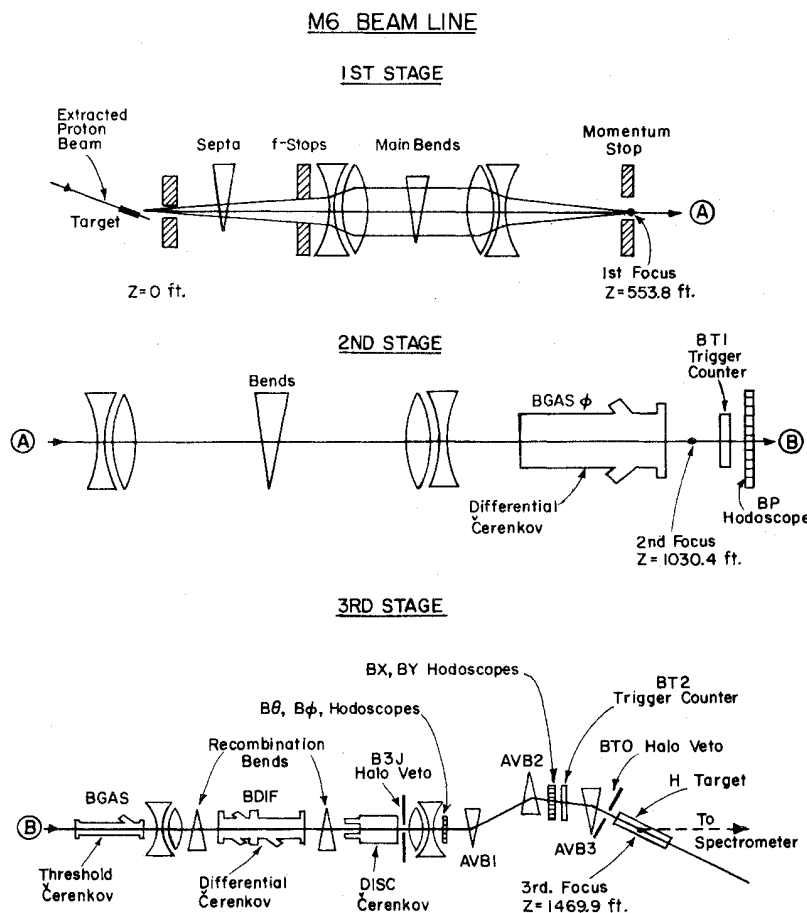
FIG. 1. The three stages of the Fermilab Meson Laboratory M6 beam line.
