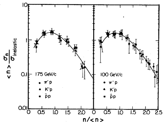
FIG. 10. KNO scaling data for negative beam, total-cross-section trigger. The curve is the KNO fit (Ref. 30) for pp \rightarrow X reactions.
