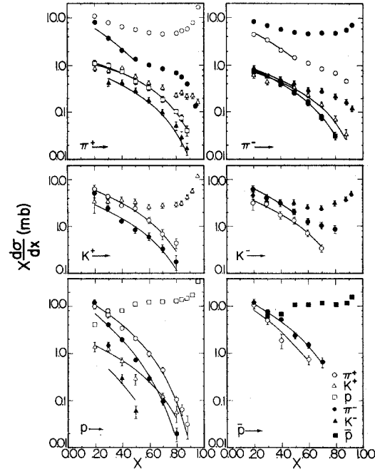
FIG. 18. The single differential cross section x d\sigma/dx is shown as a function of x . It is obtained by integrating the invariant cross section over transverse momentum. The incident energy is 100 GeV. There is one subfigure for each incident-particle type.
