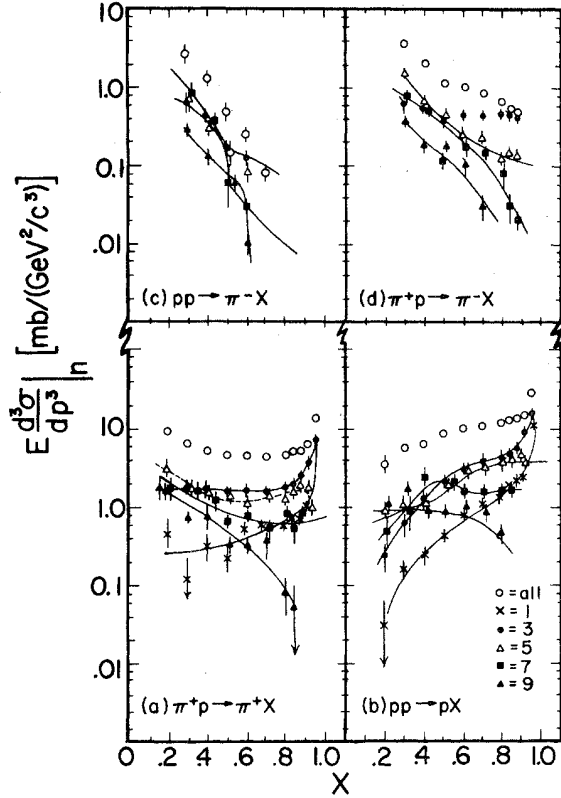
FIG. 25. Feynman- x dependence of contribution of n -prong cross sections E d^3 \sigma / dp^3 |_n for \pi^+ p \rightarrow \pi^\pm X , pp \rightarrow pX , and pp \rightarrow \pi^- X at fixed p_T .
