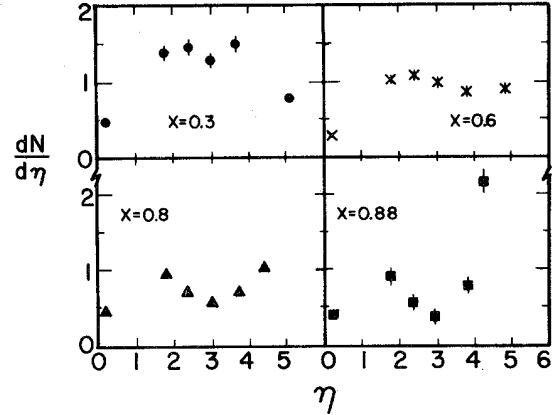
FIG. 32. x dependence of the associated pseudorapidity distribution for \pi^+ p \rightarrow \pi^- X at 100 GeV/c and p_T = 0.3 GeV/c.
