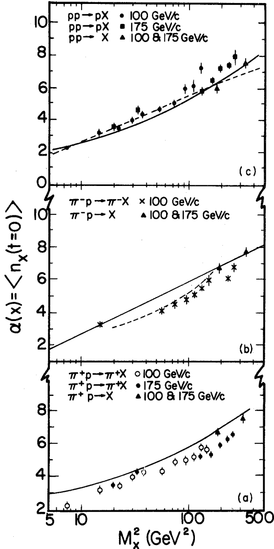
FIG. 29. Parameter \alpha(x) for fits of the form \langle n(x,t) \rangle = \alpha(x) - \beta(x)t for leading-particle \pi^\pm p \rightarrow \pi^\pm X and pp \rightarrow pX channels. Also plotted are the multiplicities for the \pi^\pm p \rightarrow X and pp \rightarrow X total-cross-section trigger of Table XI at a common s = M_X^2 . The solid curve is a parametrization of Ref. 44, for ap \rightarrow X total multiplicities. The dashed curve represents fits of Ref. 40 for ap \rightarrow aX associated multiplicities as observed in bubble-chamber experiments.
