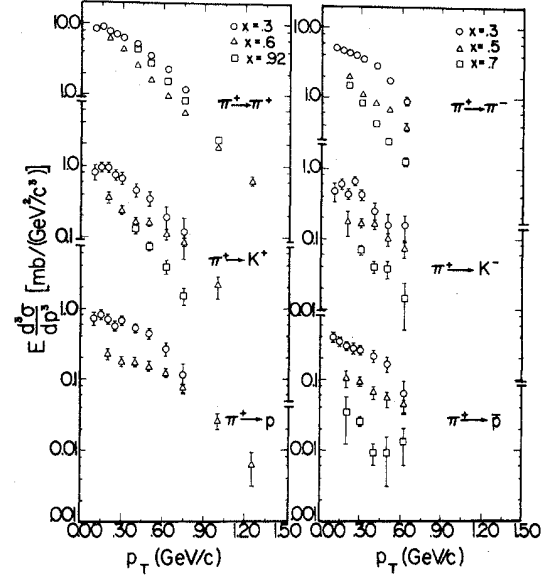
FIG. 15. The invariant differential cross section for \pi^+ -induced reactions is shown as a function of transverse momentum p_T . The incident energy is 100 GeV. The values of x for which the transverse-momentum dependence is shown are those at which the most thorough p_T sweeps were made.
