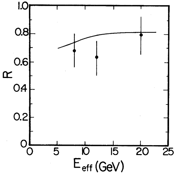
FIG. 23. The ratio R of \sigma_{\text{tot}}(K^+p)/\sigma_{\text{tot}}(K^-p) as calculated from \pi^\pm p \rightarrow K^\pm X -inclusive scattering. The curve is the \sigma_{\text{tot}}(K^+p)/\sigma_{\text{tot}}(K^-p) ratio from data of Ref. 37.
