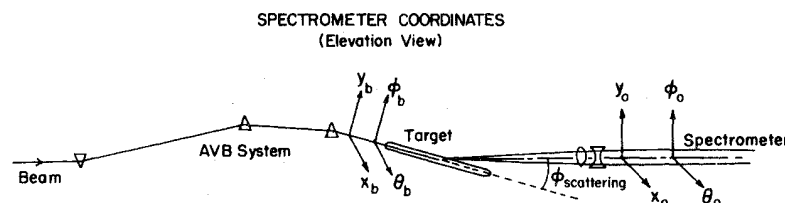
FIG. 2. The angle the spectrometer subtended relative to the incident beam direction was adjusted using an angle-varying bend (AVB) magnetic system bending in the vertical plane of the incident beam. The three magnets of the AVB are shown here in relation to the target and the spectrometer.
