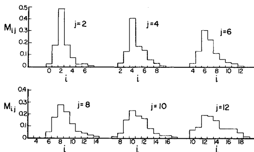
FIG. 8. Multiplicity correction matrix M_{ij} for the 100 GeV, x=0.6 , p_T=0.3 GeV/ c kinematic setting. M_{ij} represents the probability of an event with j charged prongs being detected as an event with i charged prongs as calculated by Monte Carlo methods. The efficiency for detecting the spectrometer trigger particle by the vertex detector is also included, giving j -even prong topologies.
