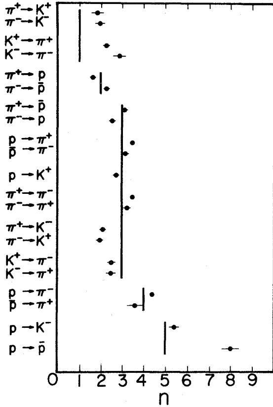
FIG. 14. The fitted exponent n for the differential cross sections fitted to the form x d\sigma/dx = C(1-x)^n . The plotted value of n represents the average for 100- and 175-GeV data runs. The vertical bars represent the values predicted by quark counting rules; see Ref. 32.
