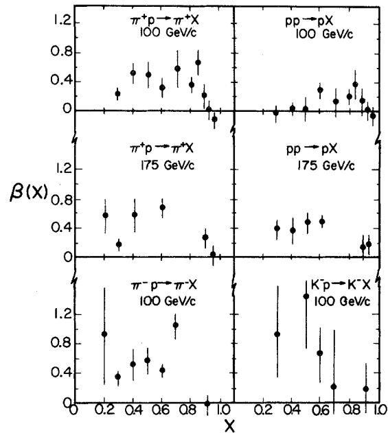
FIG. 28. Parameter \beta(x) for fits of the form \langle n(x, t) \rangle = \alpha(x) - \beta(x)t for leading-particle a + p \rightarrow a + X channels.
