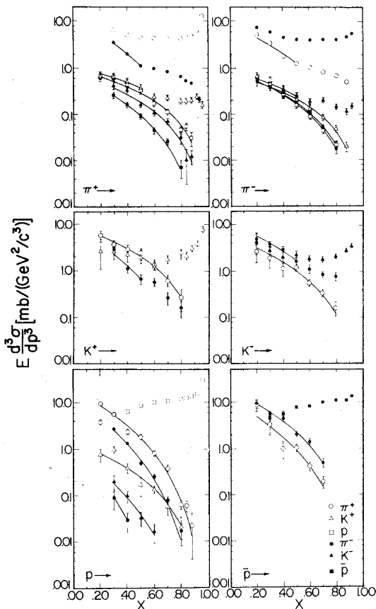
FIG. 11. The invariant differential cross section is shown as a function of x , for an incident energy of 100 GeV and a transverse momentum p_T of 0.3 GeV/c. There is one subfigure for each incident-particle type. Only those data are plotted for which the error was smaller than the value of the cross section. Comparisons to a functional form C(1-x)^n are shown.
