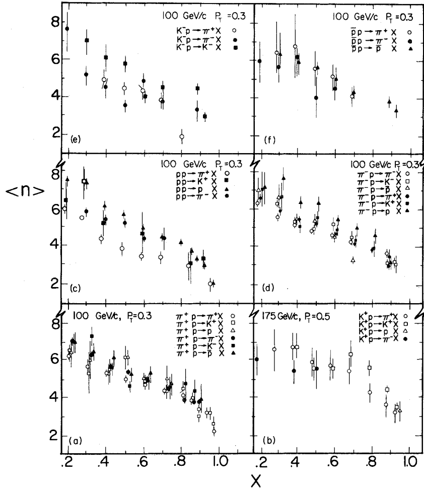
FIG. 24. Average associated-charged-particle multiplicities for a + p \rightarrow c + X as a function of x for fixed p_T .
