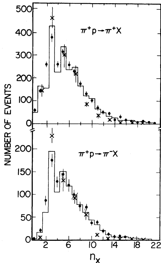
FIG. 9. Associated-charged-prong distributions n_X for \pi^+p \rightarrow \pi^\pm X at 100 GeV, x=0.6 , p_T=0.3 GeV/ c . \bullet = raw observed prong distribution N_{0i} ; \times = corrected prong distribution N_{Tj} divided by a factor of 2 to account for odd-even prong normalizations; the histogram is the fitted prong distribution \sum_j M_{ij} N_{Tj} .
