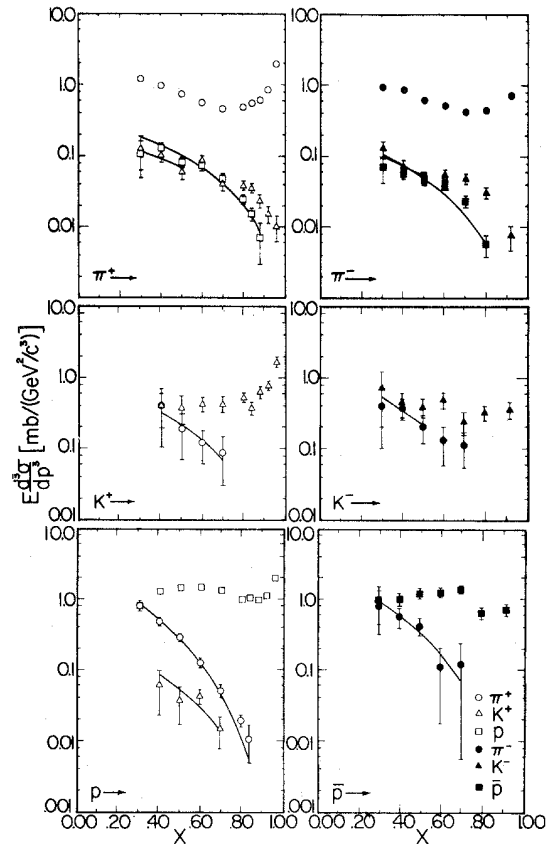
FIG. 12. The invariant differential cross section is shown as a function of x , for an incident energy of 100 GeV and a transverse momentum p_T of 0.75 GeV/c. There is one subfigure for each incident-particle type. Comparisons to a functional form C(1-x)^n are shown.
