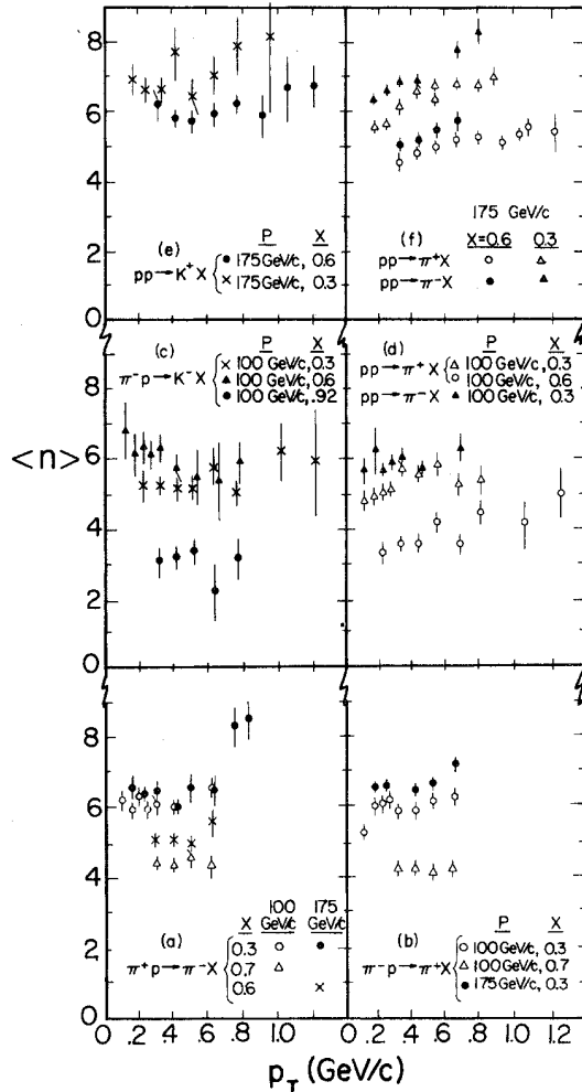
FIG. 27. Dependence of the associated-charged-particle multiplicity for particle-changing reactions a + p \rightarrow c + X on the transverse momentum of particle c at fixed x .
